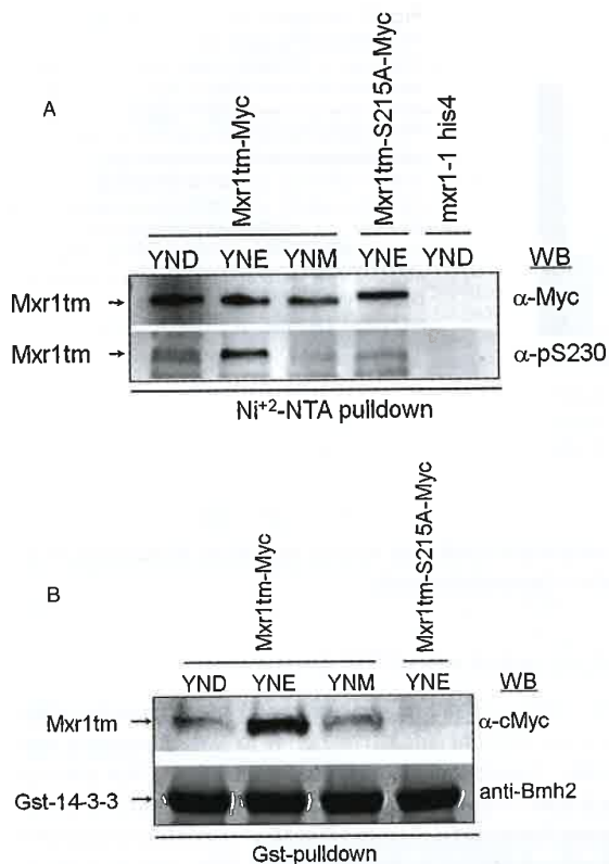
Fig. 8. A. Determination of phosphorylation of Mxr1-Ser215 in response to various carbon sources. Ni 2+ -pulldown was done using P. pastoris protein extract containing either truncated wild-type Mxr1 (Mxr1tm-Myc-His 6 ) prepared from cells grown in 0.5% glucose (YND), 0.5% ethanol (YNE) and 0.5% methanol (YNM) containing media, or truncated mutant Mxr1 (Mxr1tm-S215A-Myc-His 6 ) prepared from cells grown in 0.5% ethanol (YNE) containing media, or extract prepared from mxr1-1 null mutant strain grown in 0.5% glucose containing media (YND). Pulldown fractions were electrophoresed in 4–20% SDS-PAGE and visualized by immunoblotting with anti-cMyc and anti-pSer230 antibody. B. Interaction studies between Mxr1 and 14-3-3 in response to various carbon sources. Gst-pulldown was performed using the P. pastoris cell extracts and E. coli expressed Gst-C4qzn3 as described above. Pulldown fractions were electrophoresed in 4–20% SDS-PAGE and visualized by Western blotting with anti-cMyc and anti-Bmh2 antibody.
