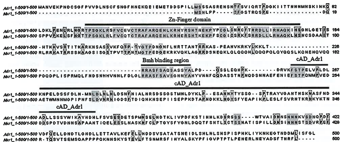
Fig. 1. Sequence alignment of Mxr1 and Adr1. The alignment was done using web server based alignment program, ClustalW2 ( http://www.ebi.ac.uk/Tools/msa/clustalw2/ ) (Larkin et al. , 2007) by taking 1–500 amino acids of both the proteins. cAD, cryptic activation domain; Zn-Finger, DNA binding domain.
