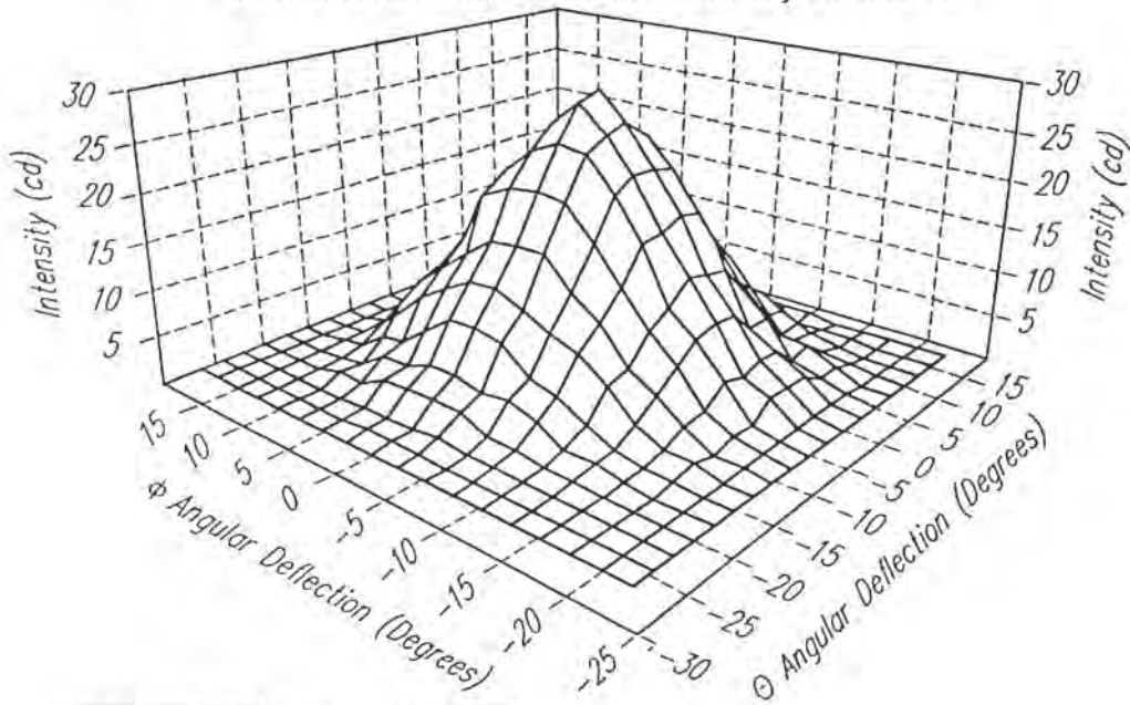
Binary-Complementary Metameric-White LED Map Light For Interior Electrochromic Mirror Initial Intensity Distribution
