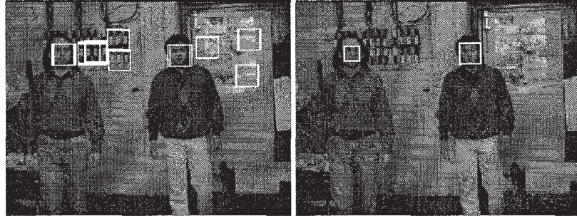
Figure 2. Left: Example output from a neural network based static face detector at a given scale. Erroneous detections occur due to “face-like” patterns. Right: Example output when the motion-based tracker and the model-based face detector are combined.
