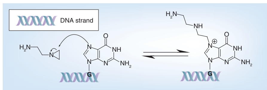
Figure 5. Reaction mechanism of binary ethylene imine with DNA or RNA (guanine).
