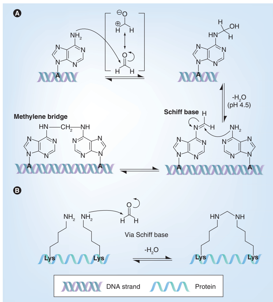
Figure 1. Reaction mechanism of formaldehyde with either DNA/RNA or amino acids. Reaction with (A) DNA or RNA (adenine) and, in a similar fashion, (B) amino acids (e.g., lysine) of proteins with a primary amine group: monohydroxy methylation and methylene bridge formation. A: Adenine; Lys: Lysine.
