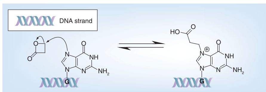
Figure 4. Reaction mechanism of \beta -propiolactone with DNA or RNA (guanine). G: Guanine.
