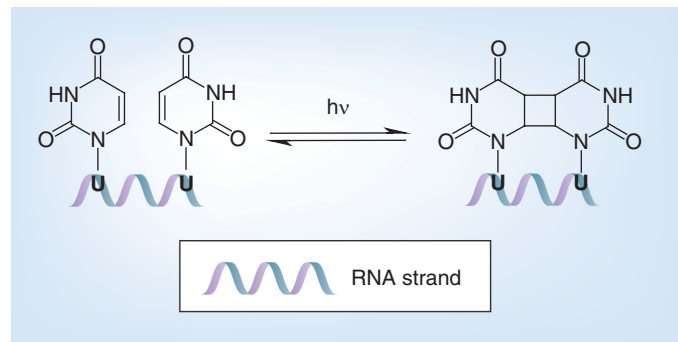
Figure 7. Ultraviolet irradiation results in pyrimidine dimer formation.
