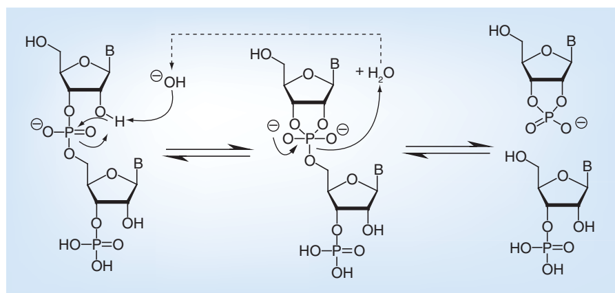
Figure 6. RNA degradation in an alkaline environment.
