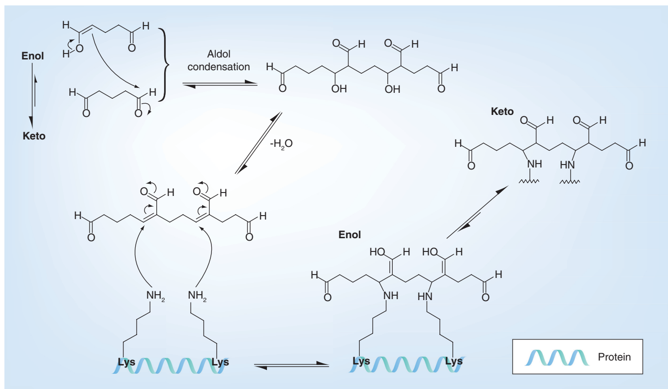
Figure 2. Reaction mechanism of glutaraldehyde with amino acids of proteins (e.g., with the primary amine group of lysine).
