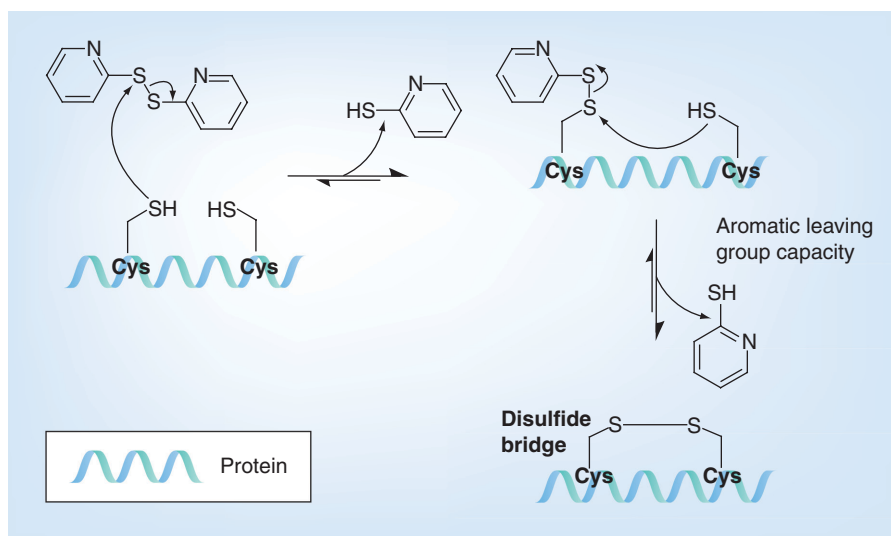
Figure 3. Reaction mechanism of 2,2'-dithiodipyridine with cysteine. Cys: Cysteine.
