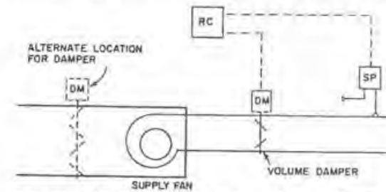
Figure 10.21 Fan volume control—volume damper. (Courtesy of ASHRAE.)
