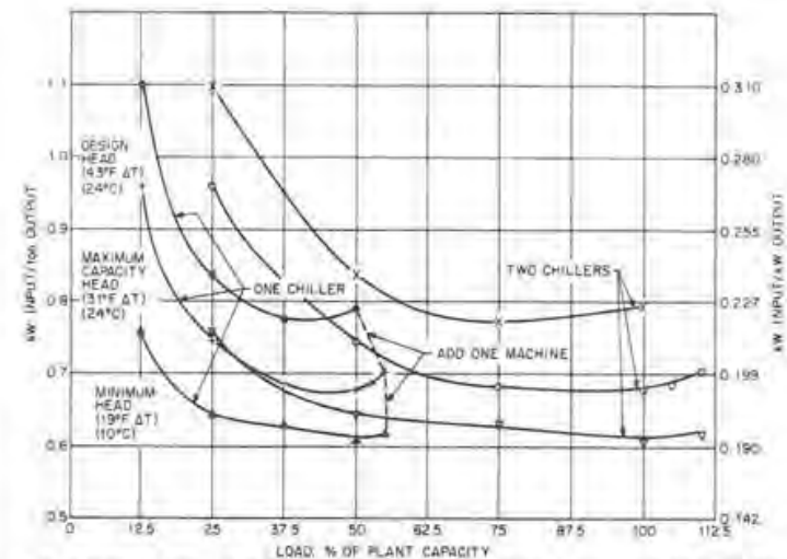
Figure 12.11 Efficiency of one or two equal-sized chillers. (Courtesy of McGraw-Hill, Handbook of HVAC Design Fig. 62.53.)
