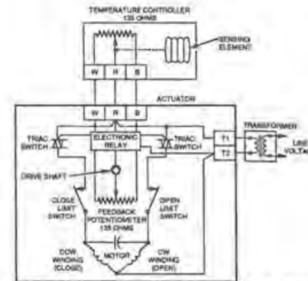
Figure 8.2 Series "90" systems. (Courtesy of Honeywell Inc.)
