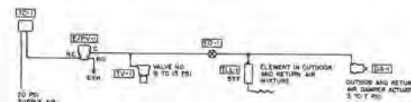
Figure 11.4 ASHRAE Cycle III. (Courtesy of Johnson Controls Inc.)
