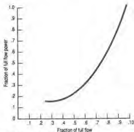
Figure 10.14 Fan horsepower versus flow.
