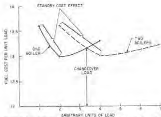
Figure 12.3 Characteristics of one versus two boilers. (Courtesy of McGraw-Hill, Handbook of HVAC Design Fig. 62.51.)
