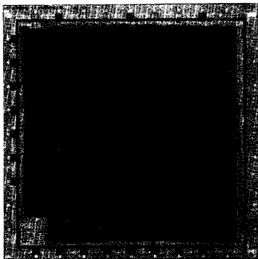
Fig. 2. Photograph of fabricated 128 x 128 CMOS APS array.
