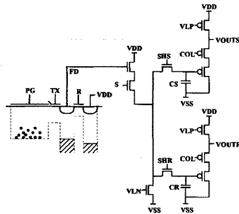
Fig. 1. Schematic illustration of image sensor circuit. Dotted line shows boundary of in-pixel circuits. The remainder of circuit is at bottom of column.
