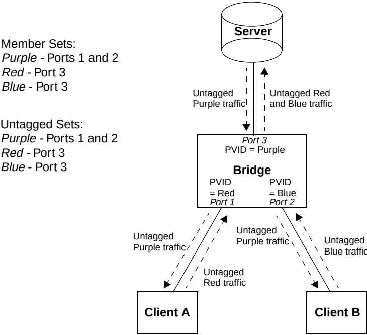
Figure B-4—Asymmetric VLAN use: “multi-netted server”
