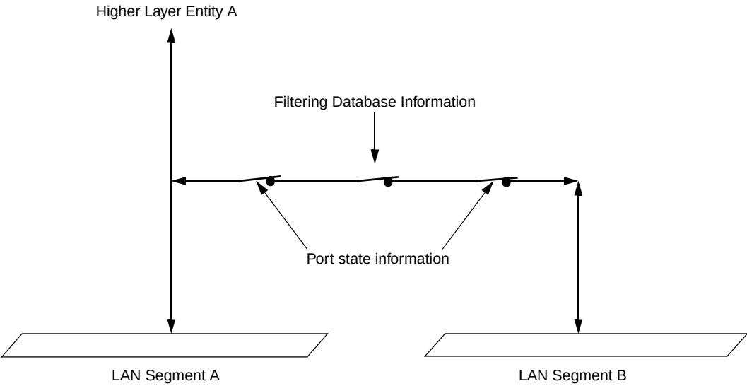
Figure 8-12—Single point of attachment—relay permitted
