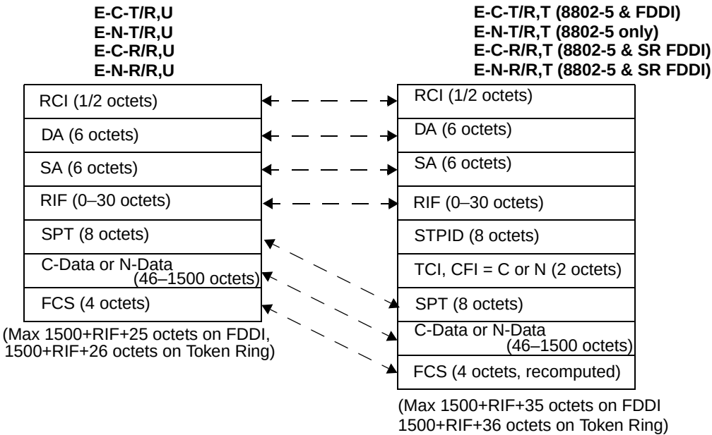
Figure C-11—Translation between E-X-X/R,U and E-X-X/R,T (8802-5 & SR FDDI)
