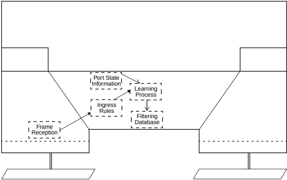
Figure 8-5—Observation of network traffic
