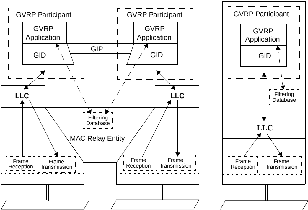
Figure 11-1—Operation of GVRP
