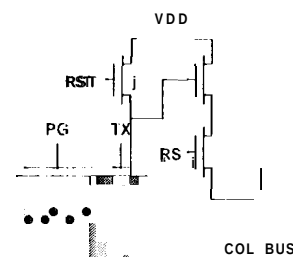
Figure 6. Photogate-type APS pixel schematic and potential wells. Transfer of charge and correlated double sampling permits low noise operation.
