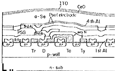
Figure 4. Crosssection of NHK CMOS APS structure with a-Si overlayer for electron bombardment from photocathode.
