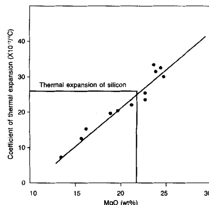
Fig. 19. Thermal-expansion tailorability in the \text{MgO-Al}_2\text{O}_3\text{-SiO}_2 glass-ceramic system.
