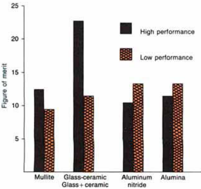
Fig. 15. Relative comparison of ceramic substrate materials.
