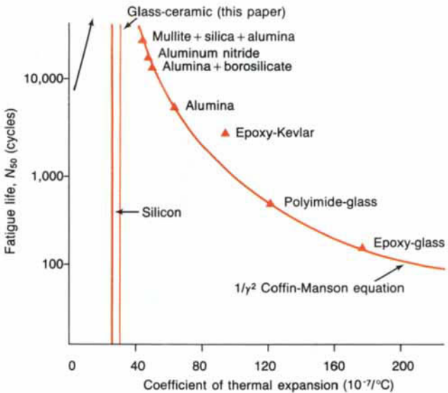
Fig. 14. Solder fatigue life improvement by glass-ceramic substrate.
