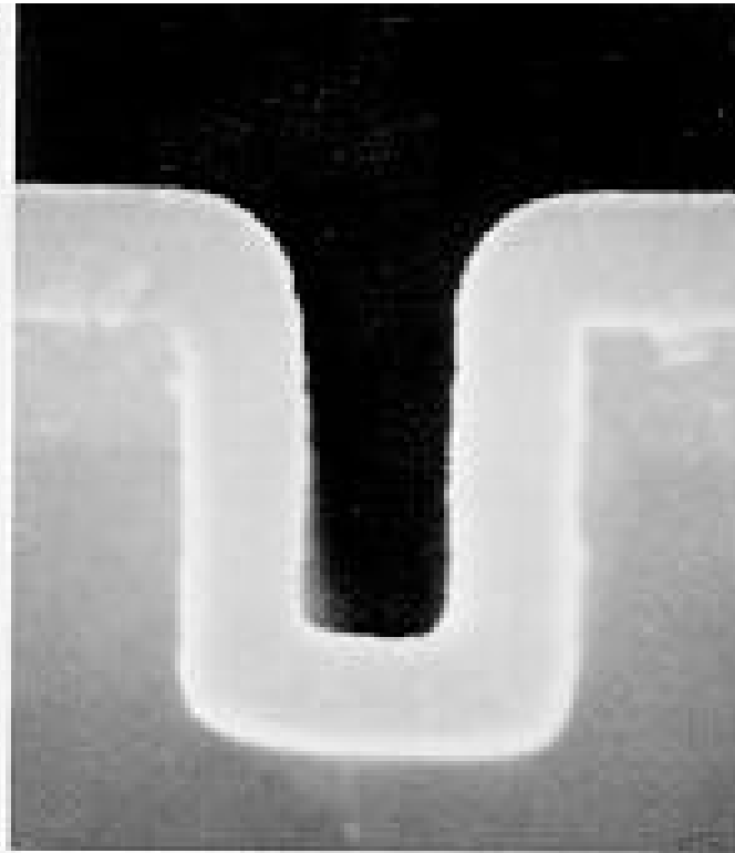
Ozone-TEOS
