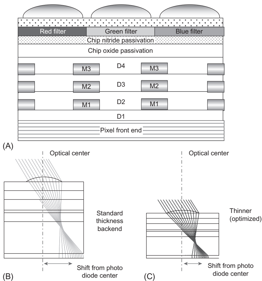
Fig. 4.2 (A) Simplified schematics of a pixel metallization backend, (B) illustration of the optical power shift for angled light rays for a standard CMOS backend, and (C) illustration of the optical power shift for angled light rays for an optimized CIS backend.
