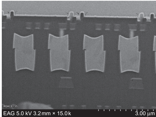
Fig. 4.17 Cross section of a wafer-to-wafer electrical test structure with 2 \mu\text{m} separation between the vias. Courtesy of Ziptronix (Huet, F. R. K., Boniface, C., Venturini, J., Ait Fqir Ali-Guerry, Z., Beneyton, R., Marty, M., Dutartre, D., 2011. High performance and high yield junction formation with full device exposure laser thermal annealing. In International Image Sensor Workshop).
