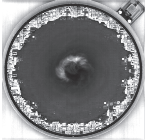
Fig. 4.11 A 200 mm P/P+ wafer after HNA etch without edge protection. The P active layer thickness is 5\ \mu\text{m} and the HNA process started after grinding of the silicon down to 20\ \mu\text{m} . At the edge of the wafer there is no active silicon left and the first inter-dielectric layer of the metallization is fully exposed.
