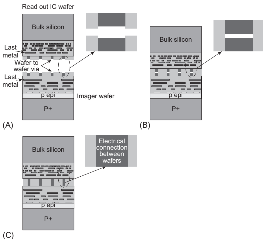
Fig. 4.16 Illustration of a typical 3D bonding between imager wafer and an ROIC wafer (A) alignment of imager wafer and ROIC wafer (each wafer surface has been prepared carefully before alignment), (B) wafers are now carefully placed one on top of the other. The surfaces of the wafers are cleaned and sometimes activated by plasma. As a result strong oxide-to-oxide bonding between the two wafers is achieved, (C) thermal treatment causes the metal to expand and create electrical connection between metals.
