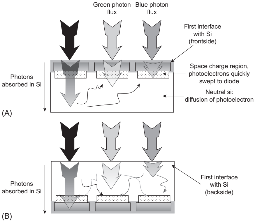
Fig. 4.6 Illustration of photon absorption in FSI pixel compared to BSI.
