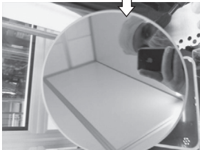
Fig. 4.12 (A) 200 mm wafer surface after HNA thinning, (B) 200 mm wafer surface after HNA thinning and CMP, and (C) X-section of the device wafer after HNA thinning showing the surface roughness.
