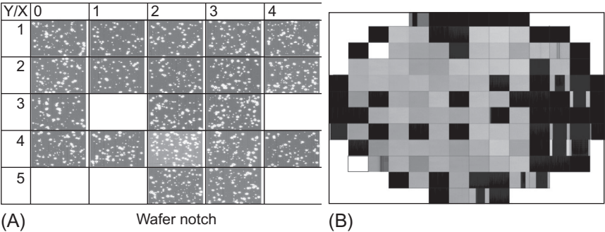
Fig. 4.7 Dark image taken from a full wafer with BSI sensor manufactured by TowerJazz (A) gray image wafer map for early process version with no proper gettering technique and (B) gray image wafer map for process which includes gettering technique.
