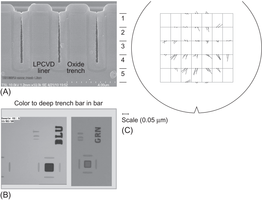
Fig. 4.14 Alignment of the color filter array to the frontend using deep trenches (A) SEM pictures of the deep trenches alignment mark, (B) blue and green color filter alignment to the deep trench mark, and (C) typical wafer map which measure the misalignment between the deep trench mark and the color filter.
