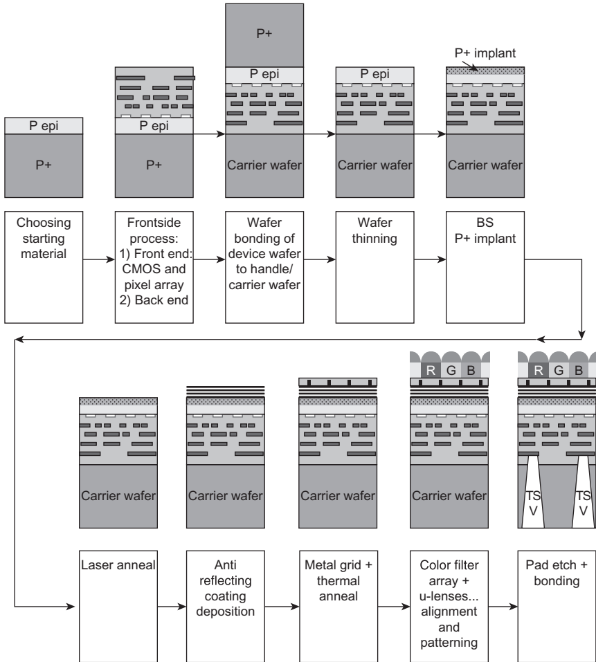
Fig. 4.5 Typical BSI complete process flow (inspired by TSMC and OmniVision from IISW 2009 (Wuu, 2009; Rhodes, 2009)).
