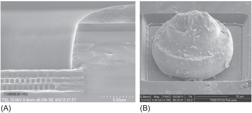
Fig. 4.15 Pad opening scheme (A) cross section showing deep etch from the sensor backside which stops at M1 of the pad structure and (B) arbitrary unit bonding in the center of the backside pad.
