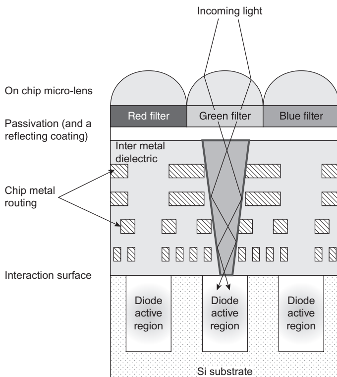
Fig. 4.3 Illustration of the light pipe concept. Deep vias etched through the inter-metal dielectric layer above each diode. The vias are filled with a slightly higher refractive index than their surroundings. The \mu -lenses are modified to ensure good coupling of the photons into the light pipe. Due to the higher refractive index in the pipe, photons are guided from the chip top surface to the diodes.
