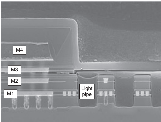
Fig. 4.4 An Aptina sensor taken from a LENOVO phone (courtesy of Chipworks, 2012 ). The sensor is fabricated using a Cu backend. There are two levels of metals in the pixel array and four levels of metals in the array periphery. In addition to the recessed backend, Aptina is using a light pipe to improve the pixel optics. The light pipe also solved the potential reflectance issue coming from the nitride-oxide-nitride interference by etching them away during the light pipe etch.
