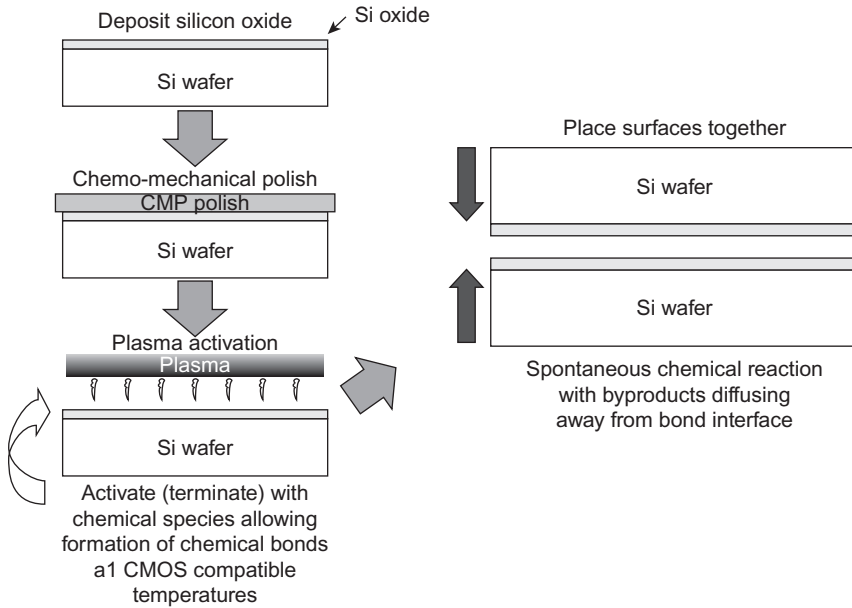
Fig. 4.8 Modern wafer-to-wafer bonding (ZiBona process flow).
