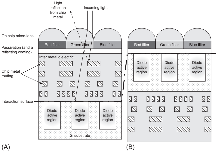
Fig. 4.1 Illustration of (A) frontside vs (B) backside illuminated sensor.
