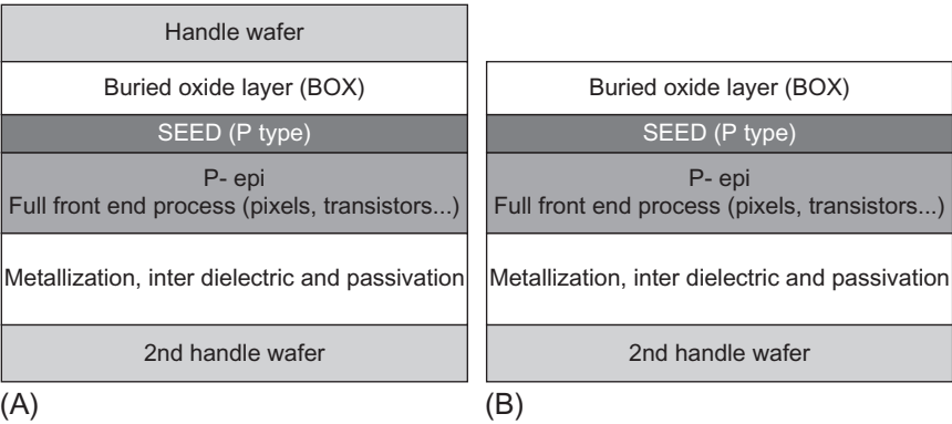
Fig. 4.9 (A) SOI wafer after wafer bonding and flipping and (B) SOI wafer after removing the first handling wafer and stopping on the SOI bottom oxide.
