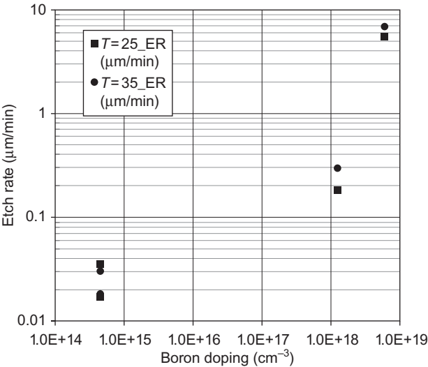
Fig. 4.10 Etch rates differences with respect to the doping level of a bare silicon wafer.
