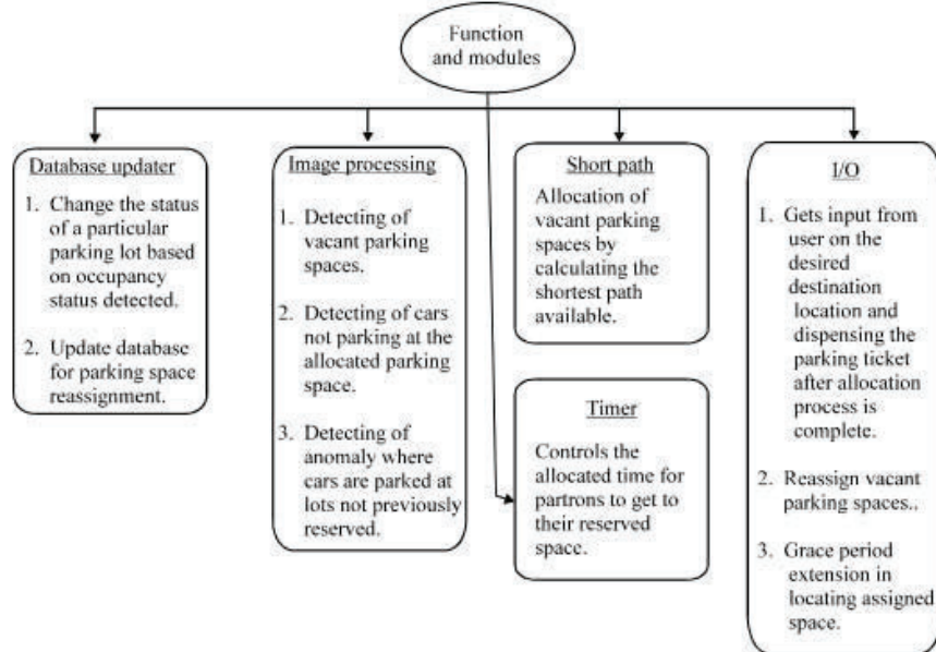
Fig. 4: Functions and modules implemented in the system
