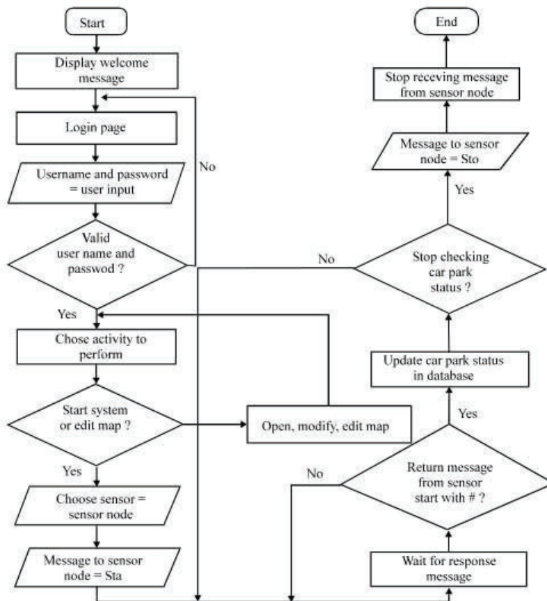
Fig. 9: Flowchart for the administrator subsystem
