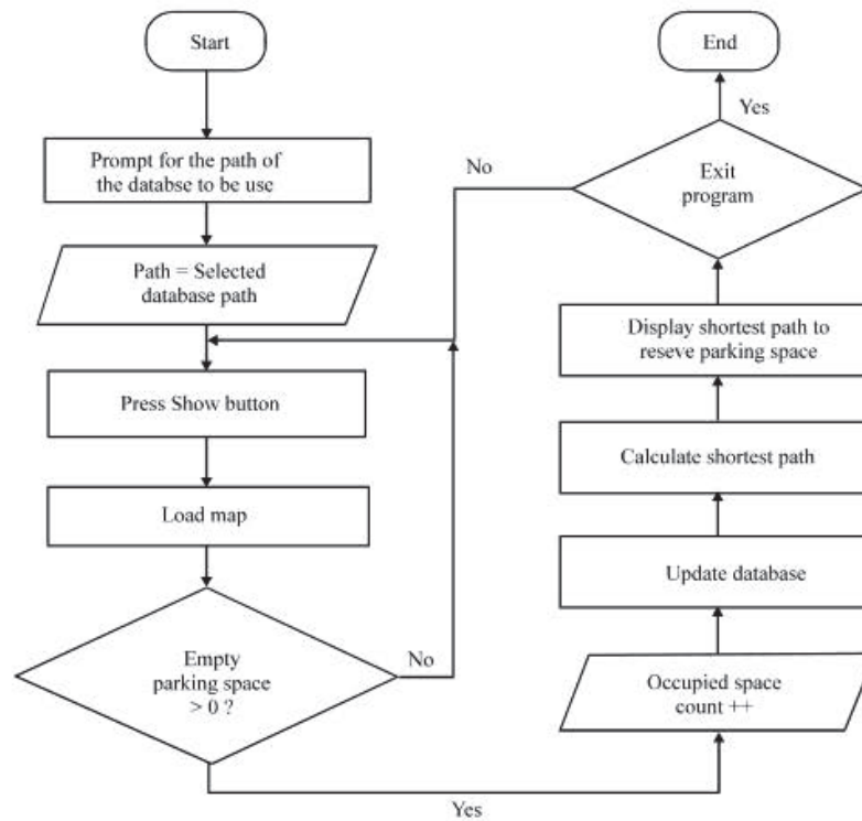
Fig. 10: Car park user subsystem
