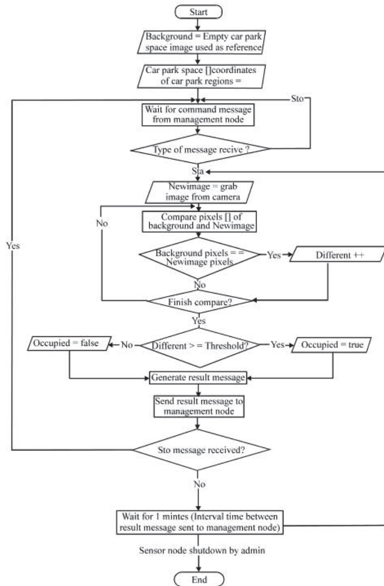
Fig. 11: Flowchart of sensor node subsystem
