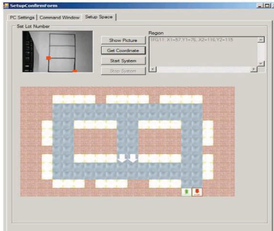
Fig. 13: The parking space coordinate region
