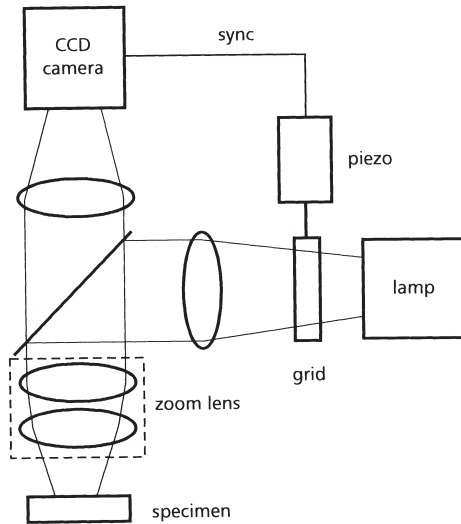
Fig. 1. Schematic diagram of the macroscope system.
