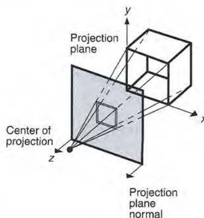
Figure 6.5 Construction of one-point perspective projection of cube onto plane cutting the z axis. The projection-plane normal is parallel to z axis. (Adapted from [CARL78], Association for Computing Machinery, Inc.; used by permission.)
