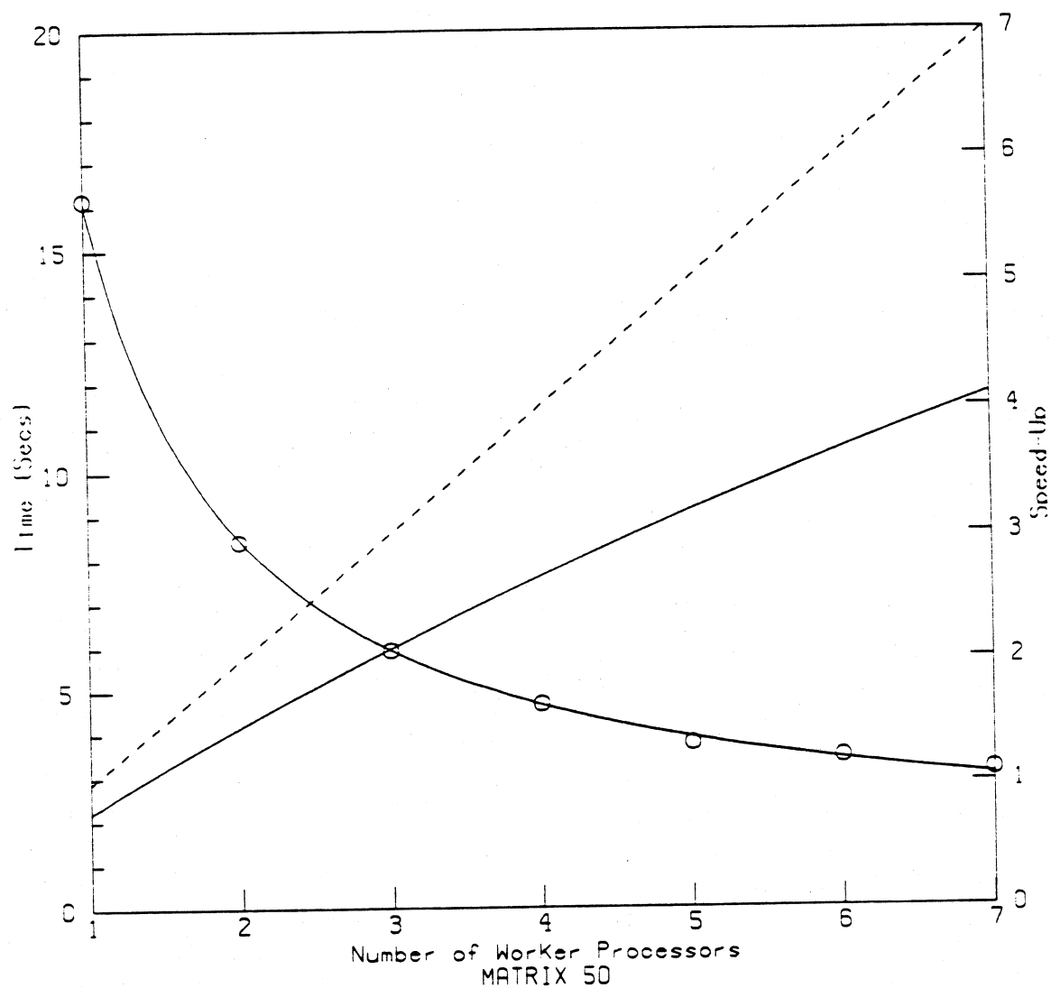
Figure 4.8: Execution time (o) vs. number of workers for a 50 x 50 matrix multiplication. Descending curve is an a/n + b model ( a = 15.29 secs; b = .83 secs). Ascending curve is speed-up relative to sequential C. Dashed line is ideal speed-up.
