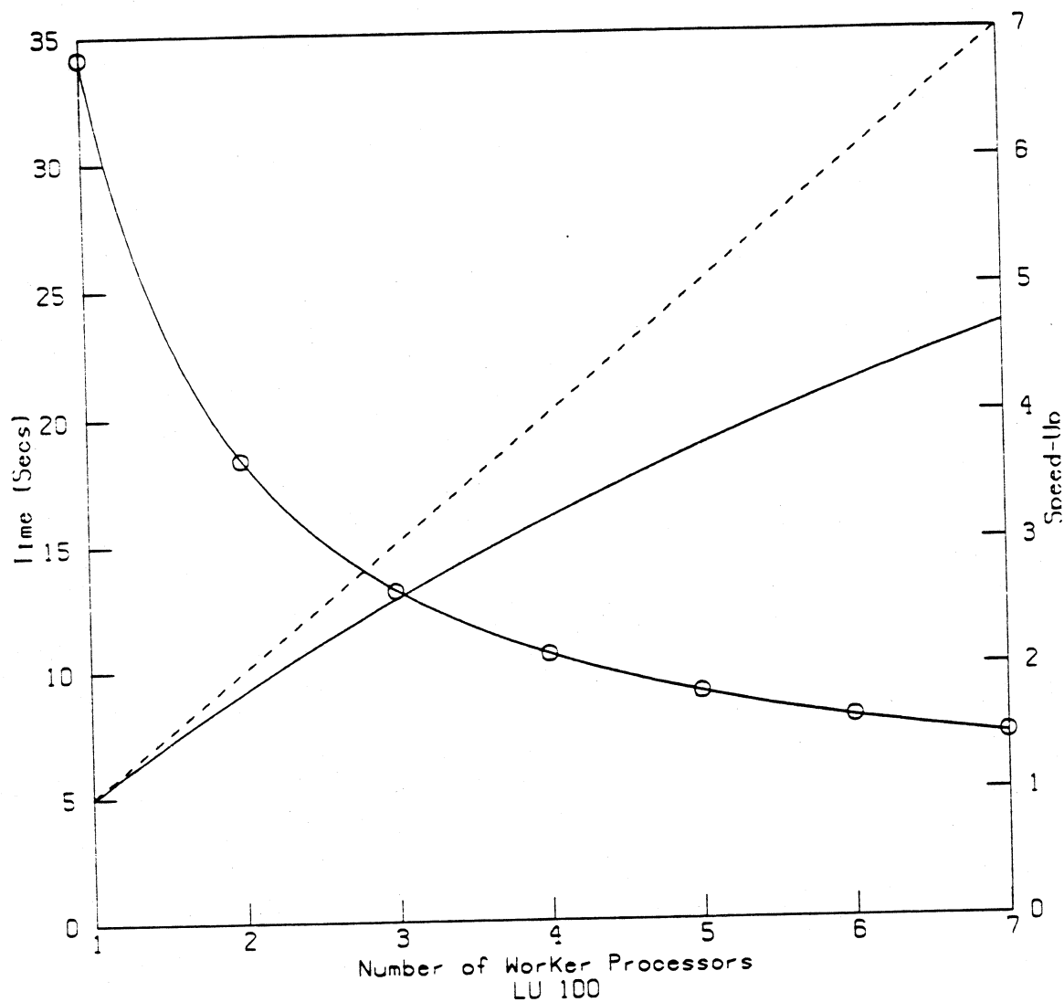
Figure 4.13: Execution time (o) vs. number of workers for the LU decomposition of a 100 \times 100 matrix. Descending curve is an a/n + b model ( a = 31.39 secs; b = 2.73 secs). Ascending curve is speed-up relative to sequential C. Dashed line is ideal speed-up.
