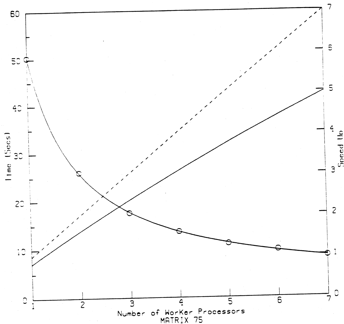
Figure 4.9: Execution time (o) vs. number of workers for a 75 \times 75 matrix multiplication. Descending curve is an a/n + b model ( a = 48.96 secs; b = 1.36 secs). Ascending curve is speed-up relative to sequential C. Dashed line is ideal speed-up.
