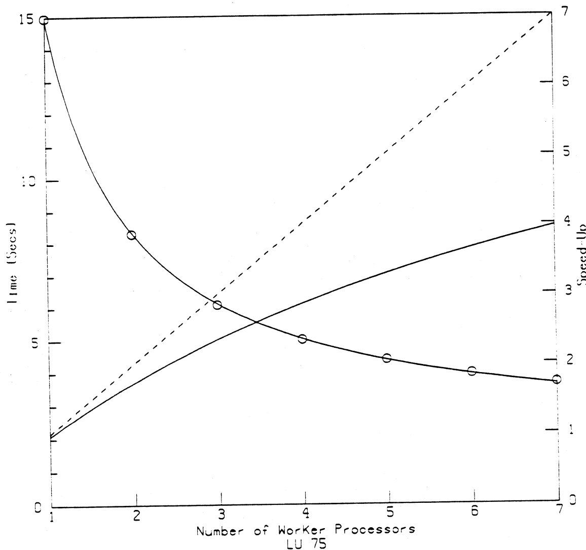
Figure 4.12: Execution time (○) vs. number of workers for the LU decomposition of a 75 \times 75 matrix. Descending curve is an a/n + b model ( a = 13.18 secs; b = 1.74 secs). Ascending curve is speed-up relative to sequential C. Dashed line is ideal speed-up.
