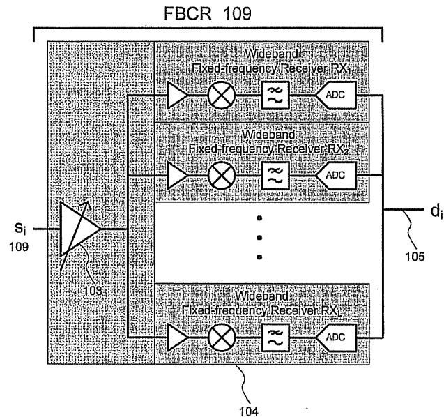
Figure 1. Broadband receiver embodiment using a multichannel approach
