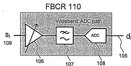
Figure 2. Broadband receiver embodiment using a full-capture approach
