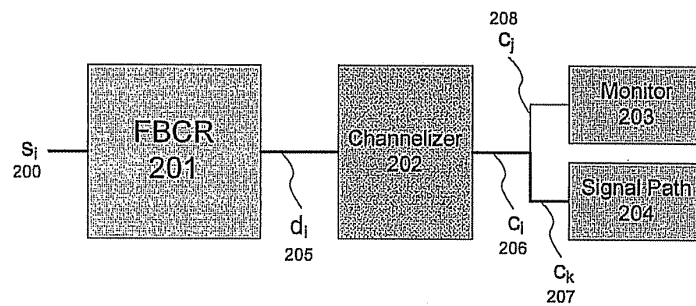
Figure 3. Embodiment of full-spectrum monitoring
