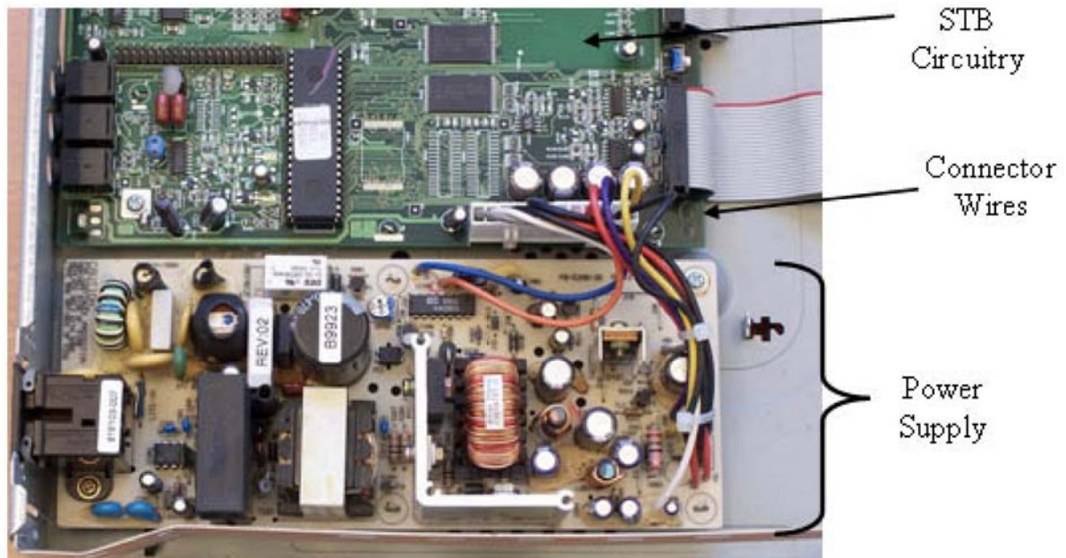
Figure 7: Typical configuration of a STB has the power supply located on a board separate from the circuitry that controls the functionality of the STB.
