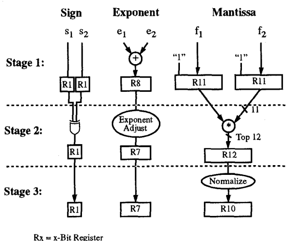
Figure 5: Three stage 18 bit Floating Point Multiplier.
