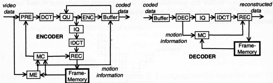
Fig. 2: Tasks and data flow of the H.263 encoder and decoder
