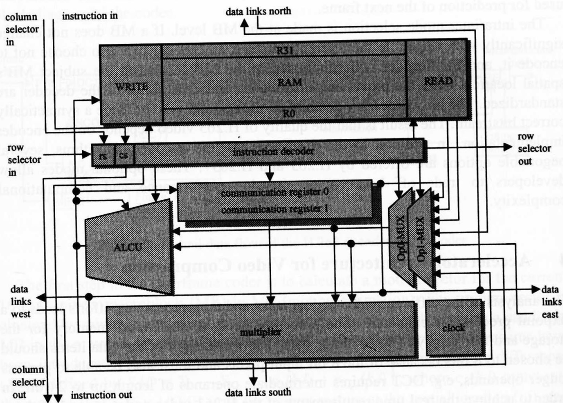
Fig. 3: Architecture of the array processor
