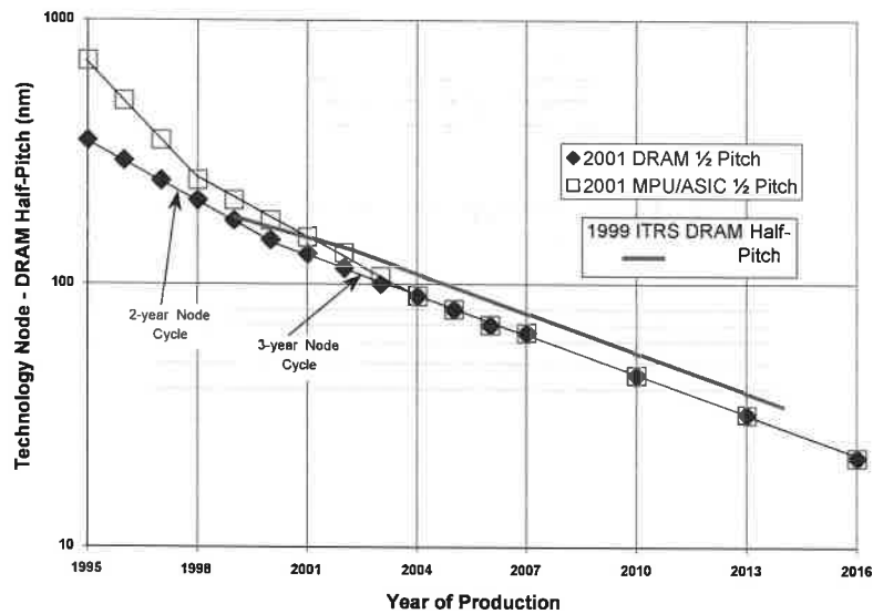
Figure 7 ITRS Roadmap Acceleration Continues—Half Pitch Trends
