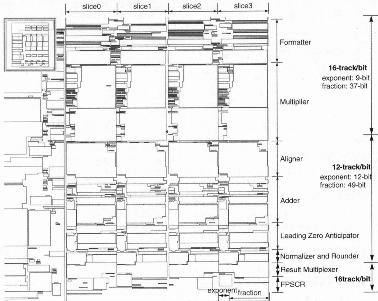
Fig. 2. Floor plan and placement of FPU macros, buffers, and stand-alone latches. Each slice has vertical dataflow of the exponent and the fraction area. There are two bit-images such as 16 track/bit and 12 track/bit.
