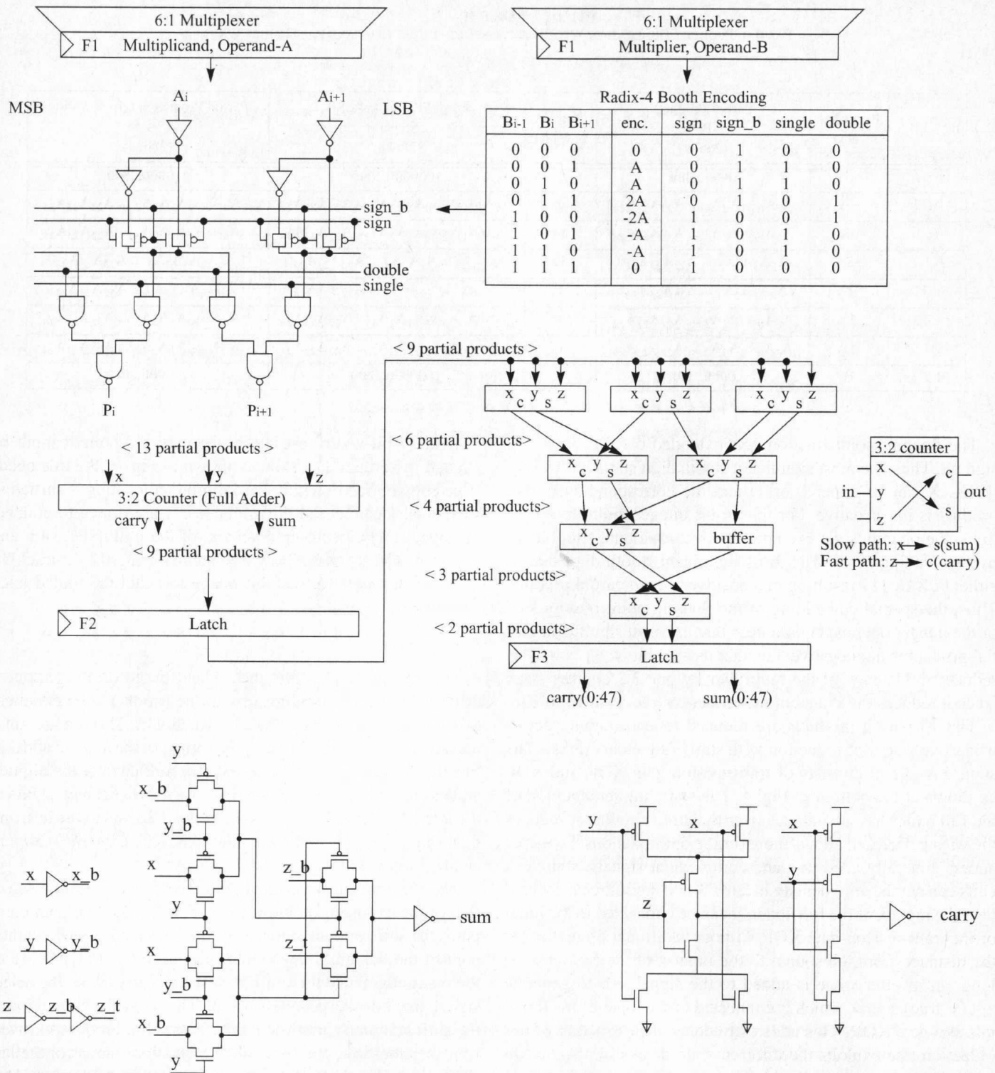
Fig. 4. Radix-4 Booth encoding table and Booth multiplexer circuits are shown. The reduction tree consists of carry-save adders. A 3:2 counter (full adder) is implemented with transmission gate and static AOI circuits.
