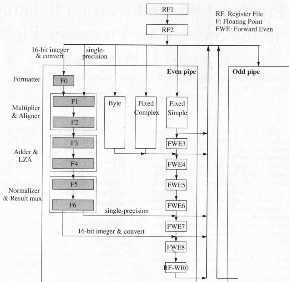
Fig. 1. Simplified pipeline structure of the floating-point unit at the SPE.
