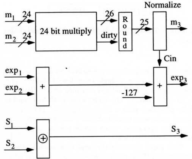
Figure 2: A block diagram of the floating-point multiplier implementation
