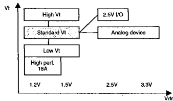
Fig. 1: Modular device portfolio of 0.13 \mu\text{m} technology platform
