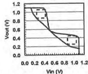
Fig.14: Measured output for the 0.157um² SRAM bit-cell with SNM 250mV.
