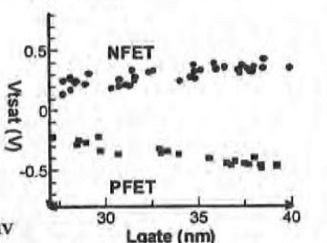
Fig.8: V_{sat} roll-off characteristics of NFET and PFET.
