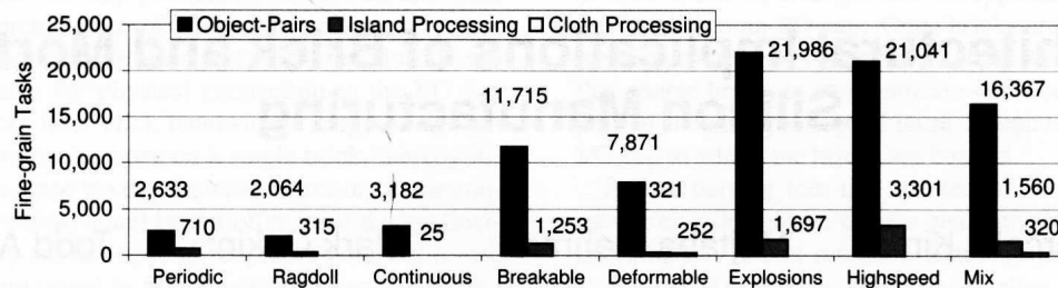
Figure 11: Average Available Fine-grain Tasks
