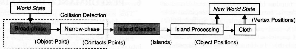
Figure 1: Physics Engine Flow.
