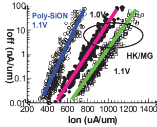
Fig.4: LSTP NFET I off -I on with 1000uA/um I on at 1nA/um I off and 1.1V V dd .
