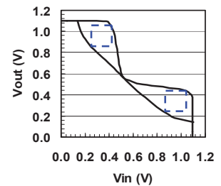
Fig.14: Measured output for the 0.157um 2 SRAM bit-cell with SNM 250mV.
