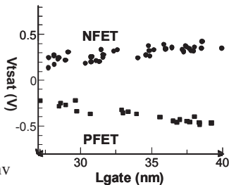
Fig.8: V i roll-off characteristics of NFET and PFET.
