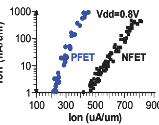
Fig.10: I off -I on of the LOP transistors at 0.8V.
