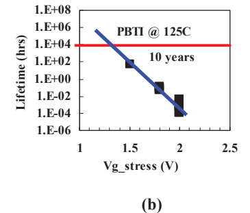
Fig.16: NBTI (a) and PBTI (b) measurements of HK-MG wafer meet 10 year lifetime requirement.
