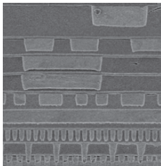
Fig.2: SEM cross-section through BEOL wiring of SRAM. First 9 layers of copper metal are shown where 7 are in ULK dielectric.
