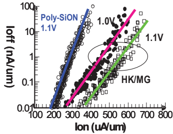
Fig.5: LSTP PFET I off -I on with 575uA/um I on at 1nA/um I off and 1.1V V dd .
