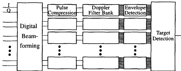
Figure 9: Description of one mode of operation in the 64-channel ground based radar system.
