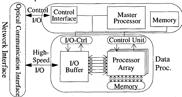
Figure 2: A Compute Engine.
