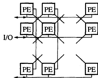
Figure 3: A 32-by-32 SIMD mesh processor array.
