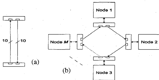
Figure 12: (a) Bi-directional fiber-ribbon link. (b) Unidirectional ring network.
