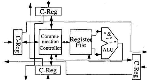
Figure 7: A bit-parallel PE.
