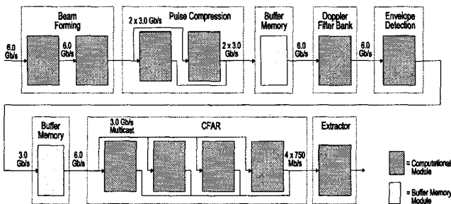
Figure 10: Allocation of link bandwidth and functions to the processing nodes.
