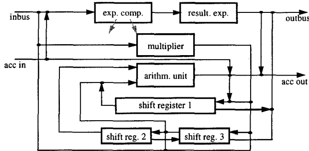
Figure 6: A bit-serial floating point PE.
