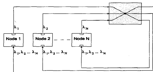
Figure 11: WDM network cluster.
