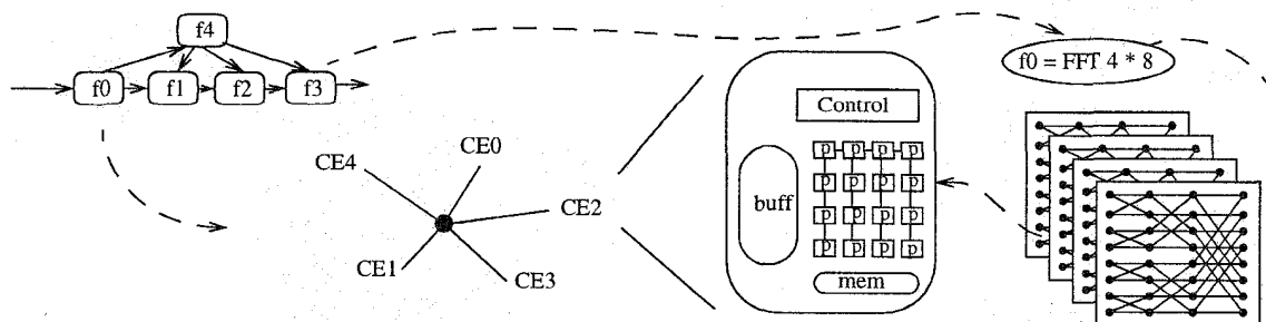
Figure 8: The MIMD system enables a functional decomposition and allocation of the program to the modules. Each function or block of functions is then mapped onto the processors 4 in the module.
