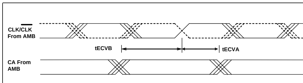
Figure 4.4 — t_{ECVA} and t_{ECVB} Timing Diagram
