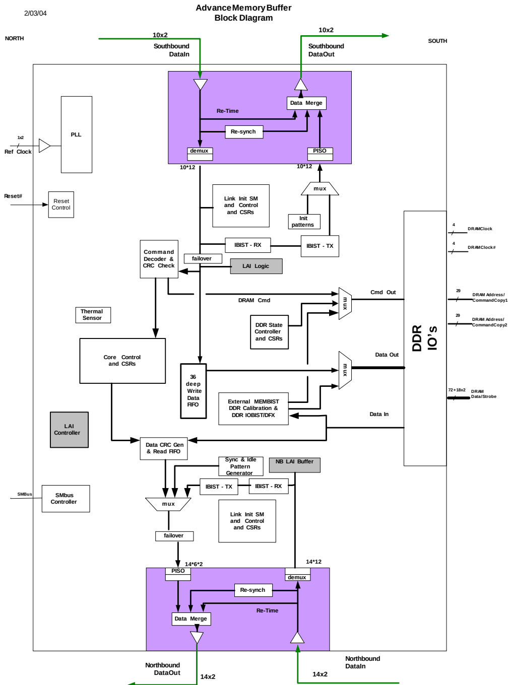
Figure 1.1 — Advanced Memory Buffer Block Diagram
