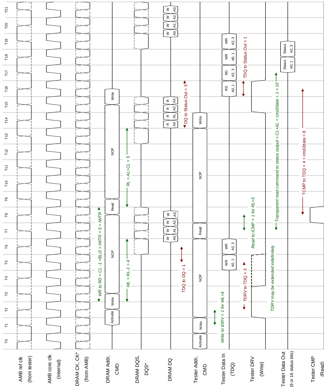
Figure 6.2 — Transparent Mode Timing
