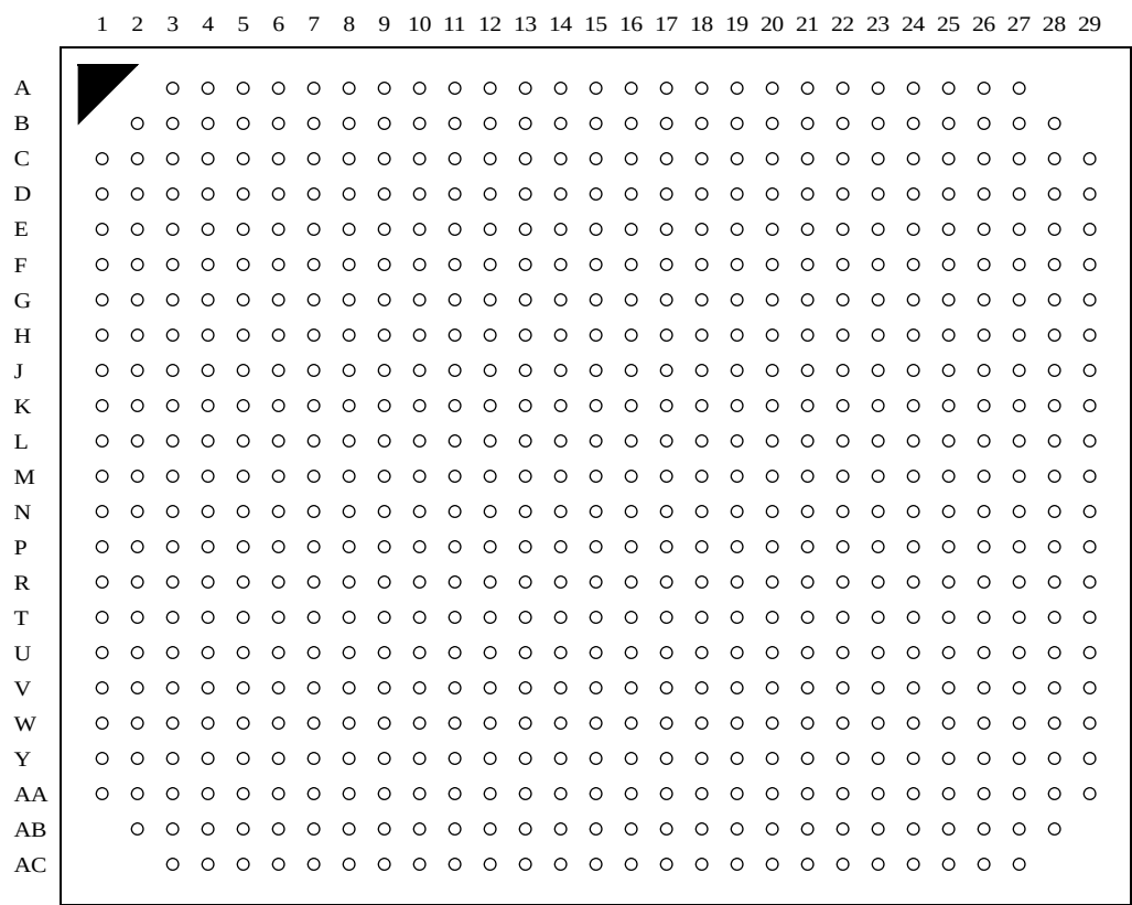
Figure 12.1 — Pinout Configuration
