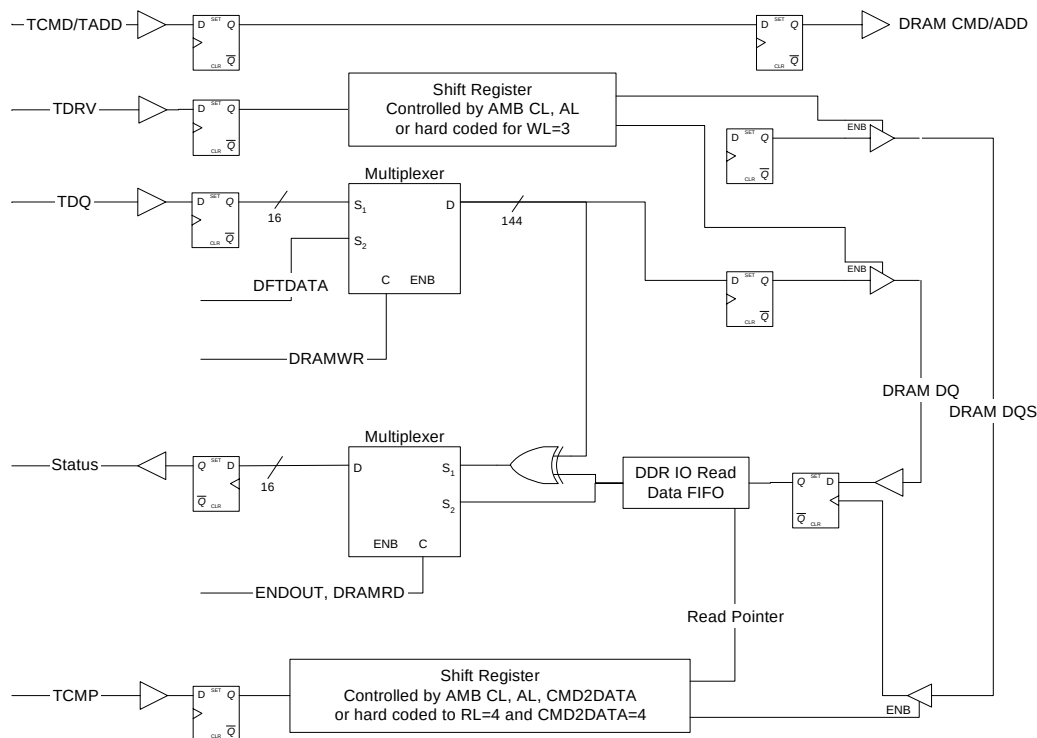
Figure 6.1 — Transparent Mode Simplified Block Diagram
