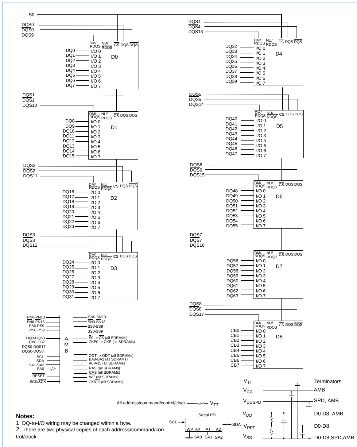
Block Diagram: Raw Card Version A (x72 ECC DIMM, one physical rank of x8 DDR2 SDRAMs)
