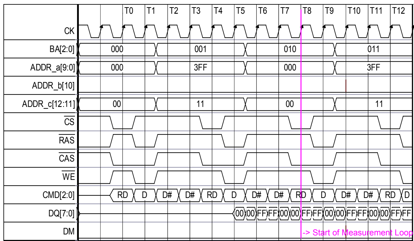
Figure 100 — IDD4R Example (DDR3-800-555, 512Mb x8): data DQ is shown but the output buffer should be switched off (per MR1 bit A12="1") to achieve I out = 0mA. Address inputs are split into 3 parts.
