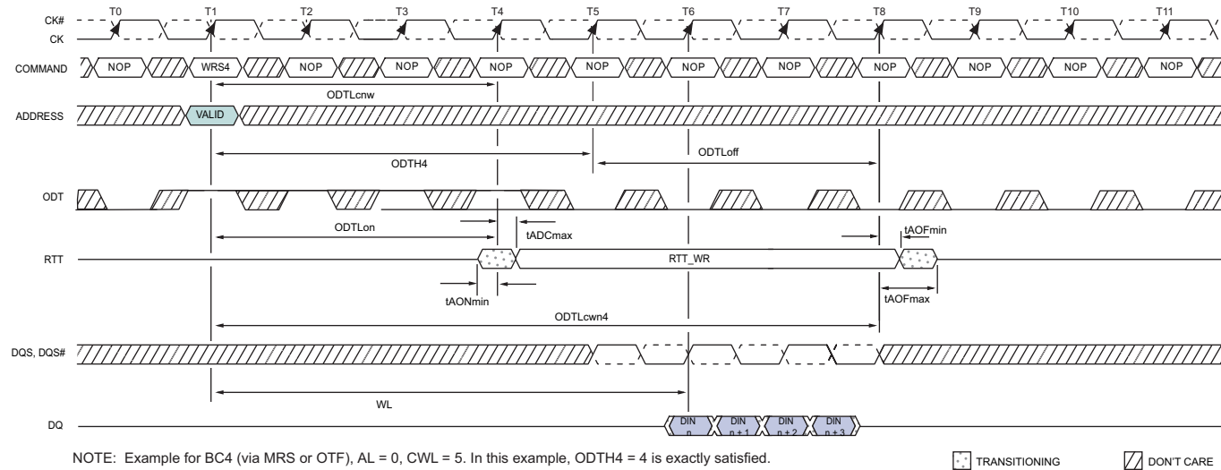
Figure 73 — Dynamic ODT: Behavior with ODT pin being asserted together with write command for a duration of 4 clock cycles
