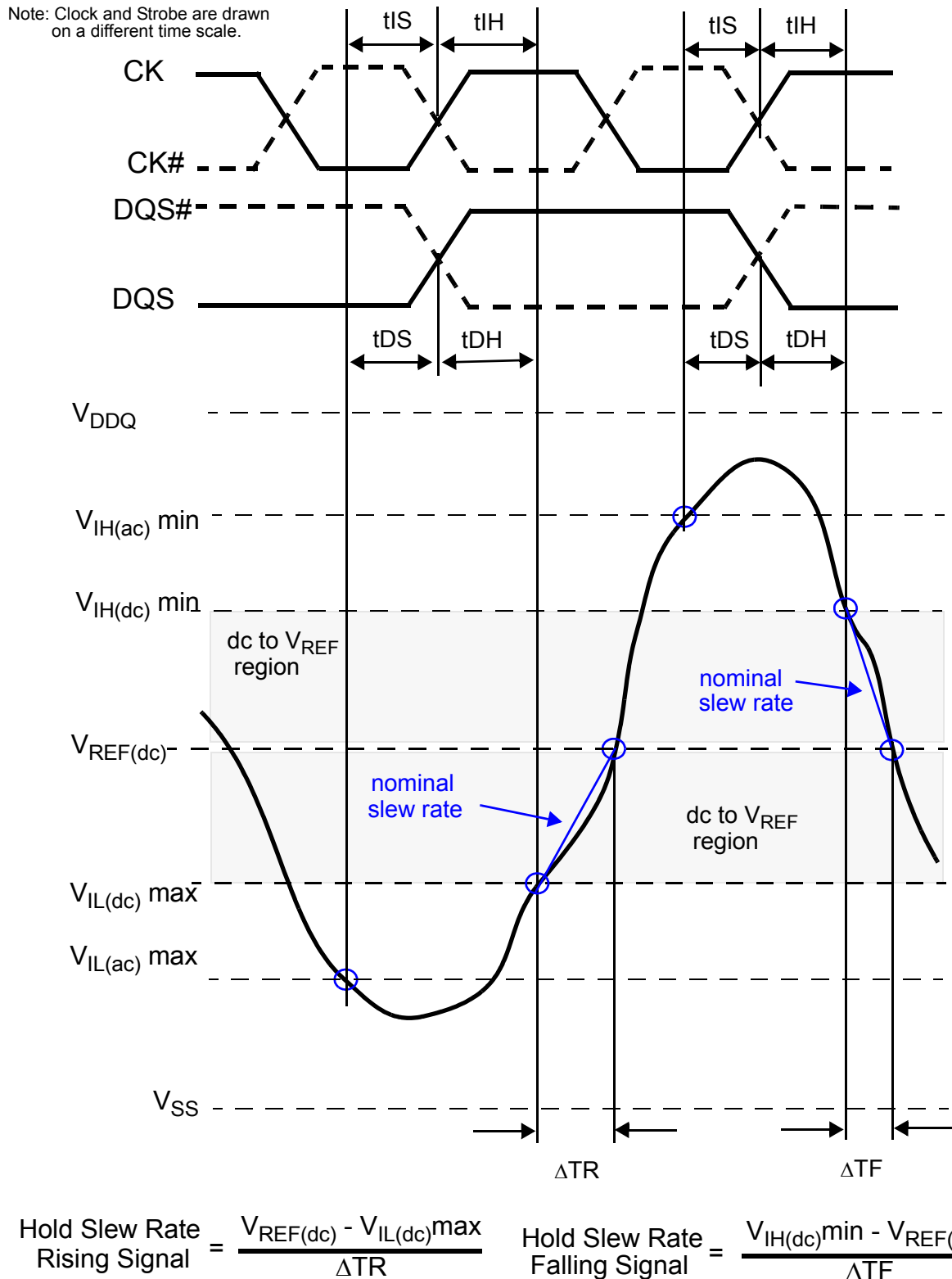
Figure 102 — Illustration of nominal slew rate for hold time t_{DH} (for DQ with respect to strobe) and t_{IH} (for ADD/CMD with respect to clock).
