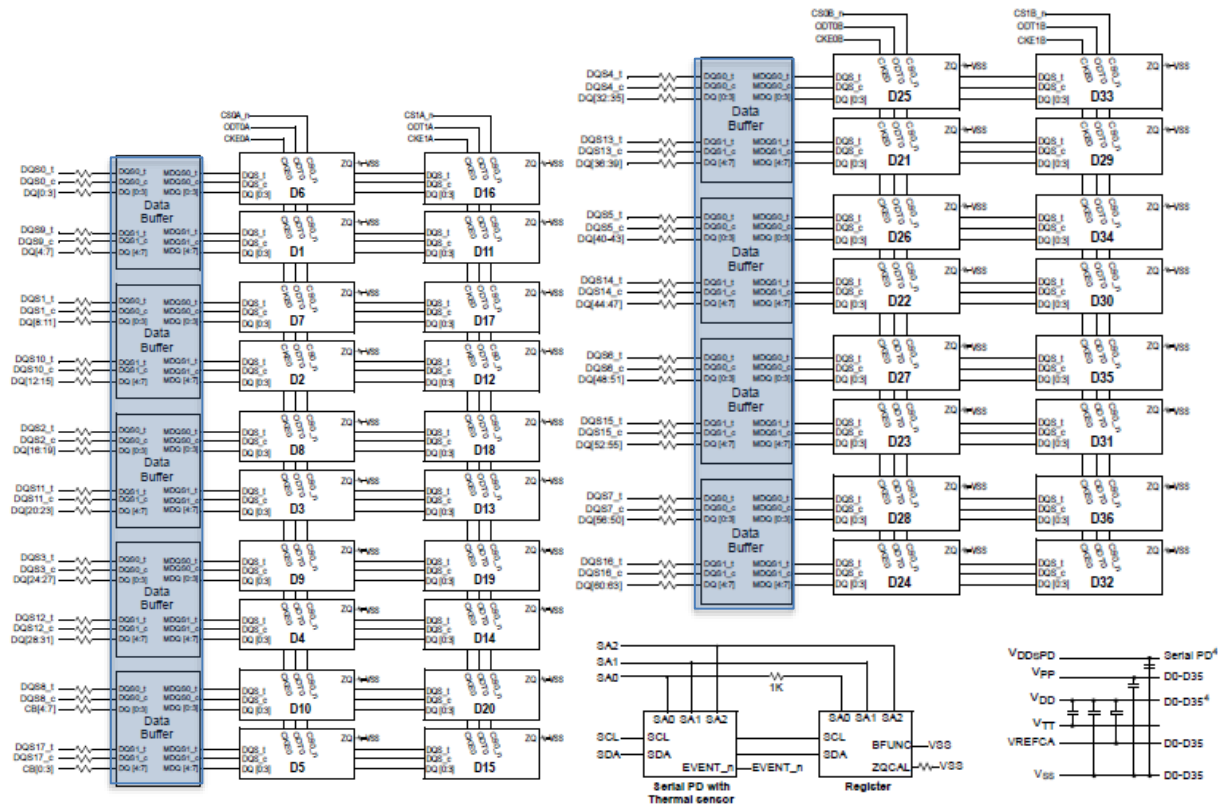
Ex. 7 (M386AAK40B40 Datasheet) at 11-12 (annotated to illustrate plurality of byte-wise buffers).
