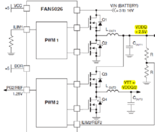
Figure 2. Typical Application
