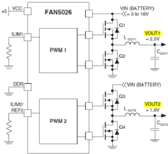
Figure 1. Dual Output Regulator
