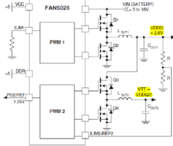
Figure 2. Typical Application
