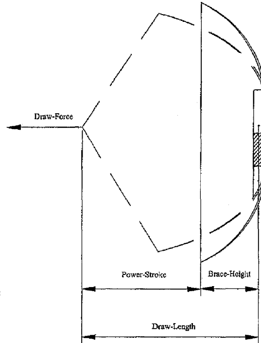
Bow Dimensions
