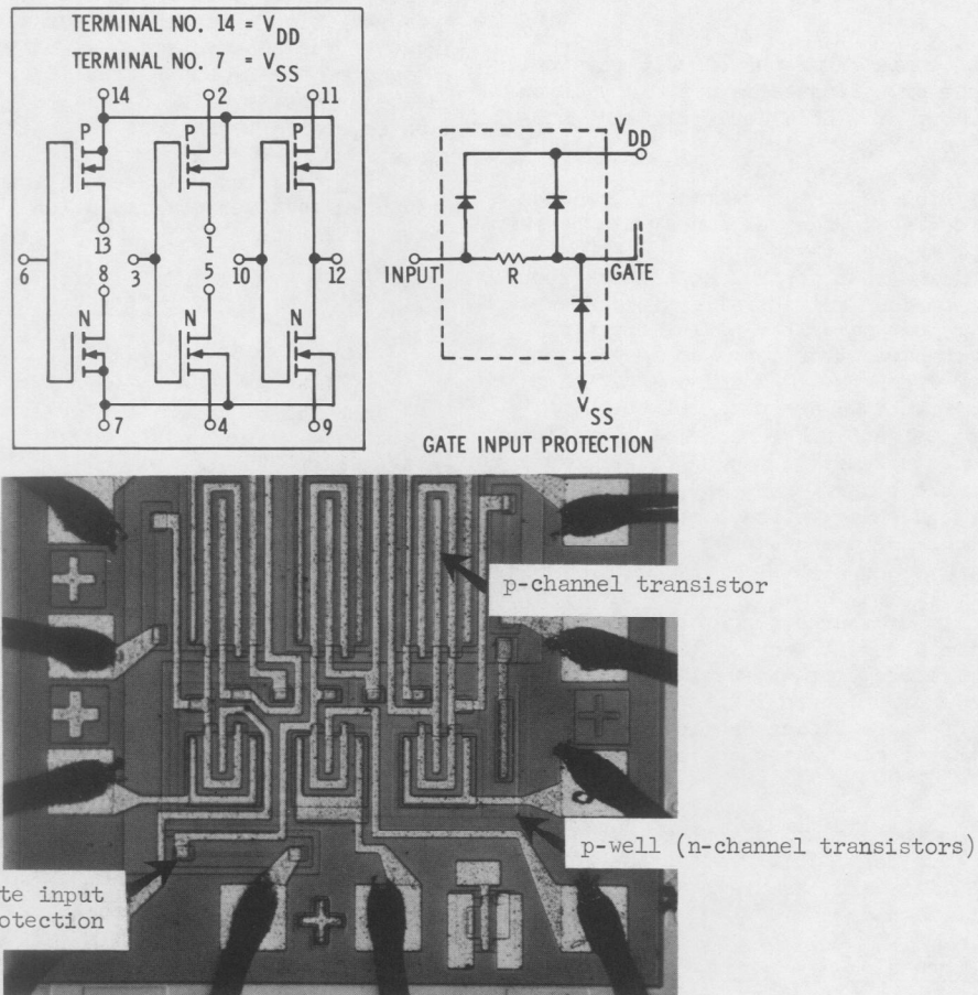
Figure 2. Layout and Schematic for the RCA CD4007A CMOS Integrated Circuit.
