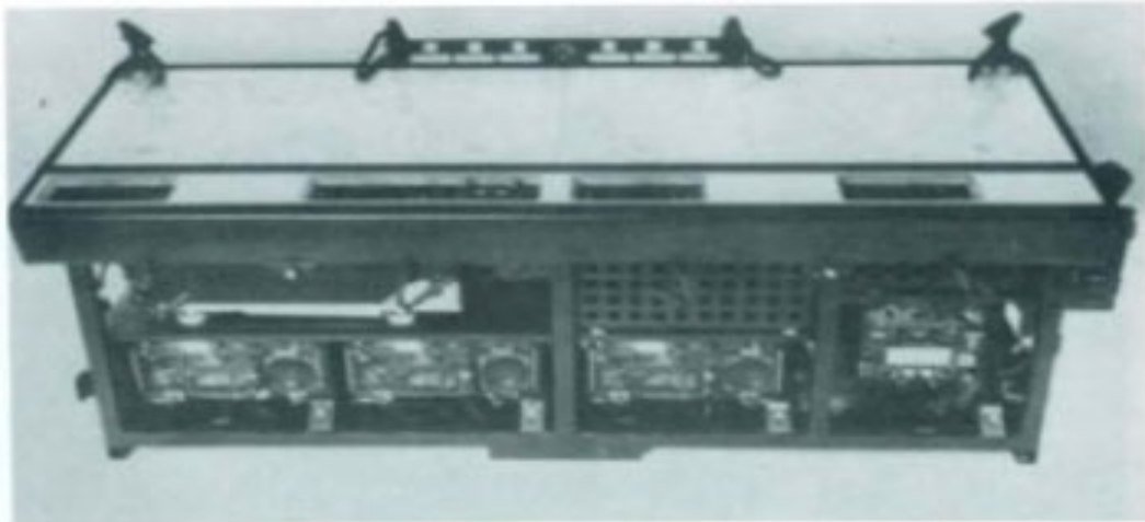
EARLY COMMAND COMMUNICATIONS CONSOLE with VRC-12 series radios.
