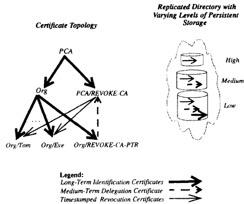
Figure 1. Experimental Revocation Architecture
