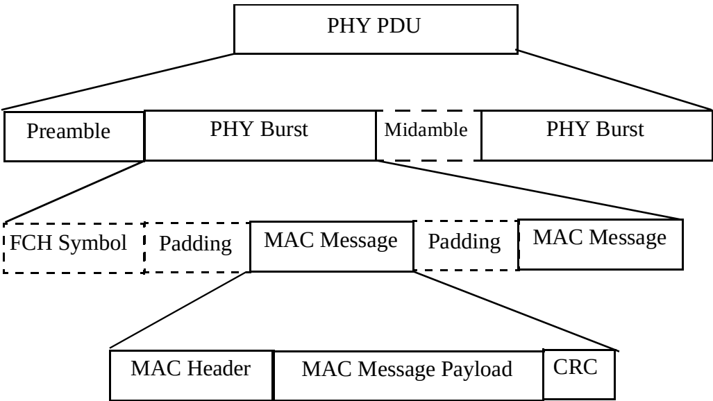
Figure 150—Burst structure
