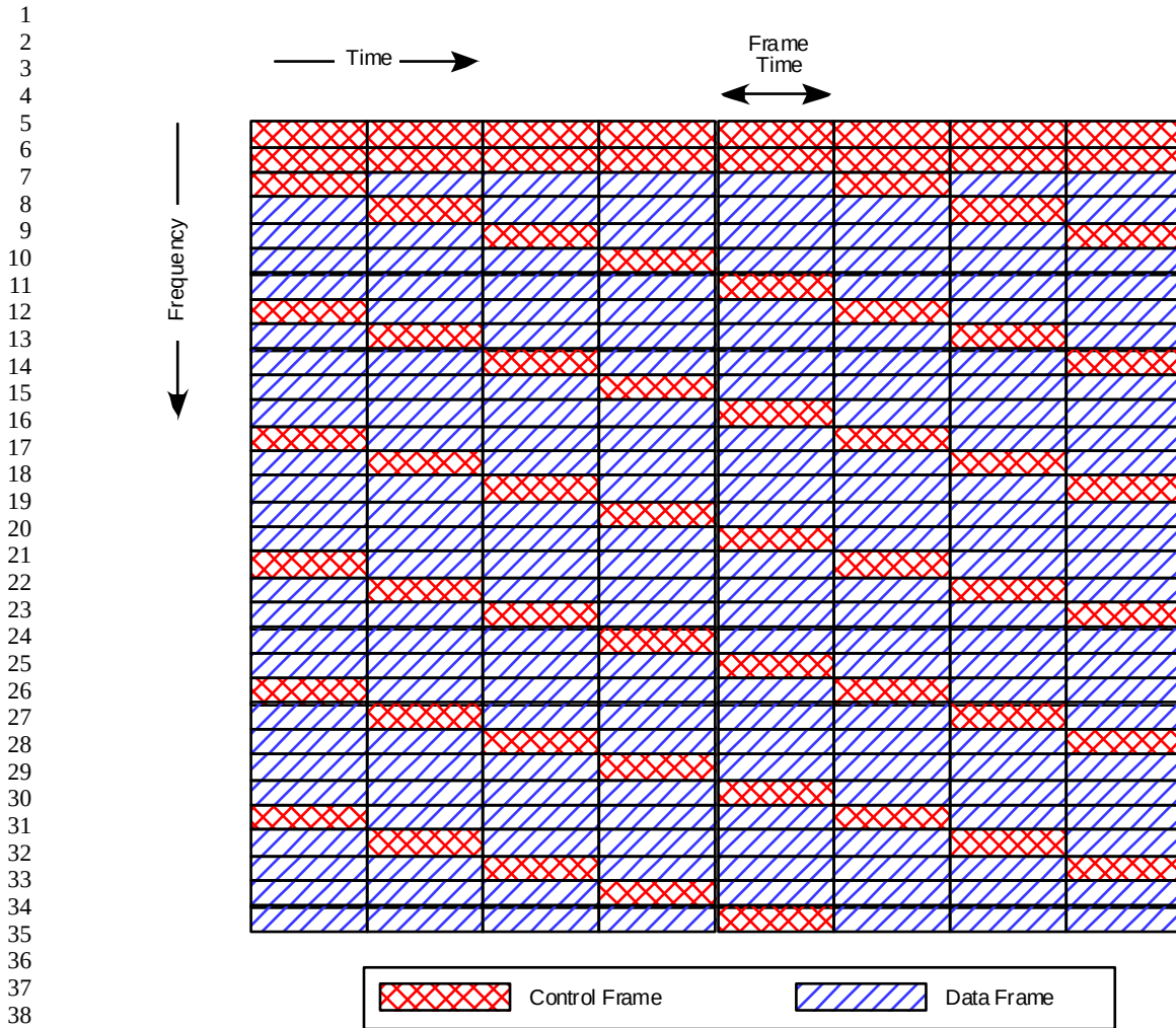
Figure 240—Superframe Layout
