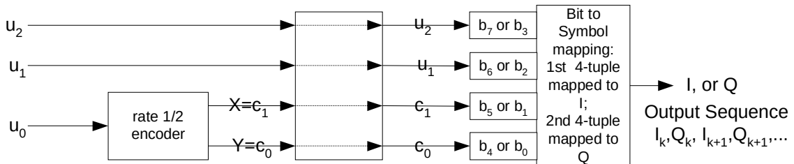
Figure 189—Optional pragmatic TCM encoder for rate \frac{3}{4} 256-QAM
