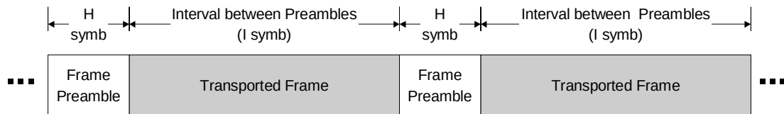
Figure 196—Frame Preamble
