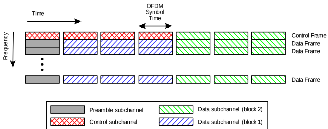
Figure 236—Downlink Framing, using Mode B Framing
