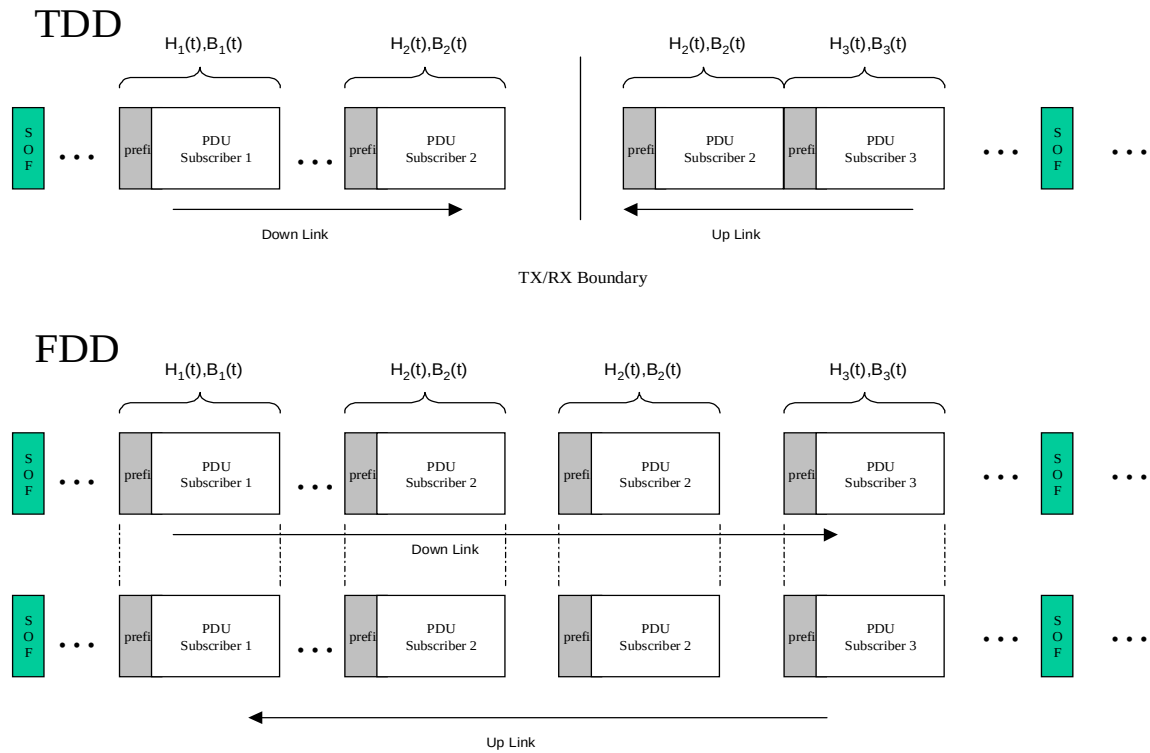
Figure 265—Beamforming Concept for TDD and FDD
