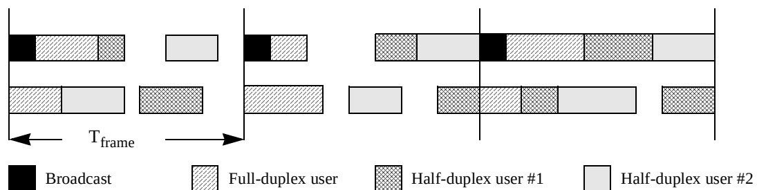
Figure 138—Example of burst FDD Bandwidth Allocation
