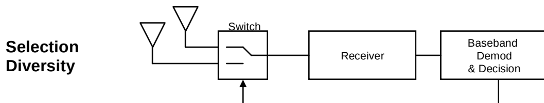
Figure 261—Selection Diversity Receiver
