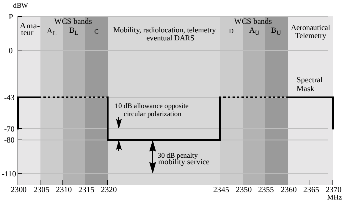
Figure 168—WCS spectral mask
