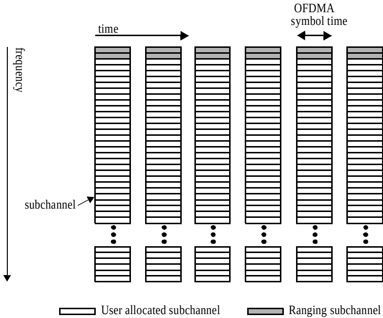
Figure 158—Ranging subchannel allocation, method #2
