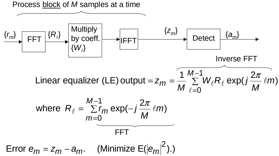
Figure 179—SC-FDE with Linear Equalization - Details
