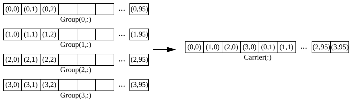
Figure 224—Symbol Interleaver for 512 FFT
