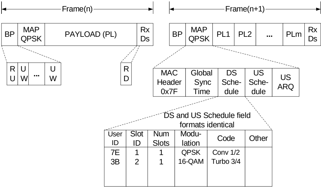
Figure 207—Burst FDD Downstream Frame
