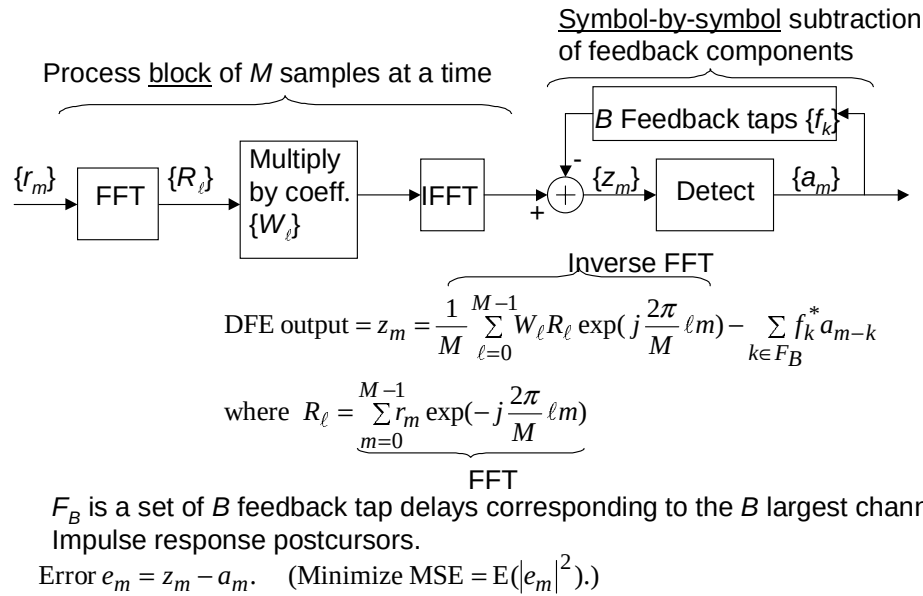
Figure 180—SC-FDE with Decision Feedback Equalizer (FD-DFE)
