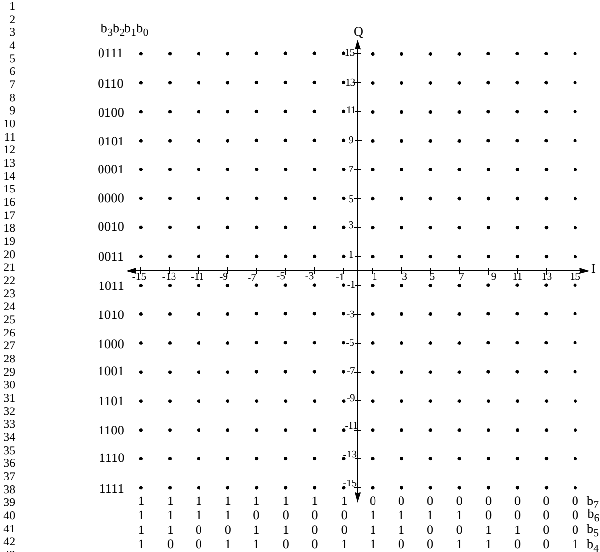
Figure 192—Pragmatic constellation map for 256-QAM
