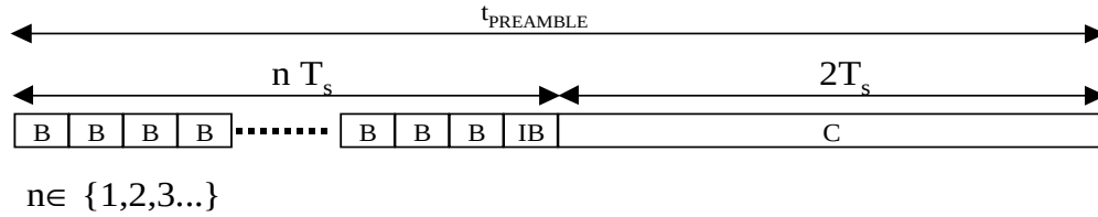
Figure 242—Complete Preamble Structure
