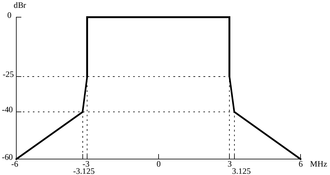
Figure 169—MMDS spectral mask
