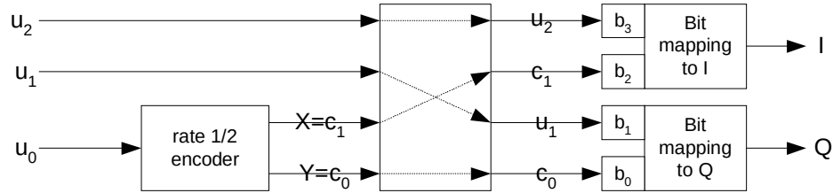
Figure 186—Pragmatic TCM encoder for rate 3/4 16-QAM
