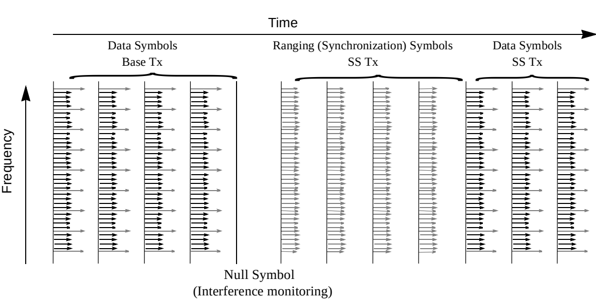
Figure 157—Ranging symbol allocation, method #1, (TDD mode)
