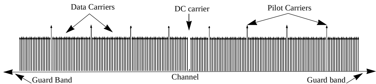
Figure 214—OFDM frequency description (256-FFT example)
