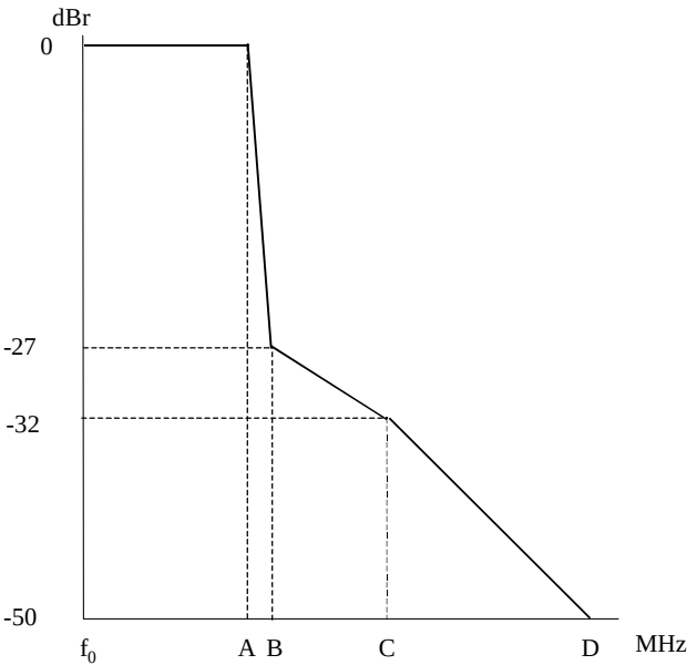
Figure 245—Transmit Spectral Mask (see Table 226)
