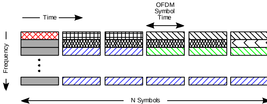
Figure 235—Downlink Framing
