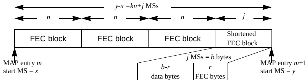
Figure 140—DL-MAP usage and shortened FEC blocks
