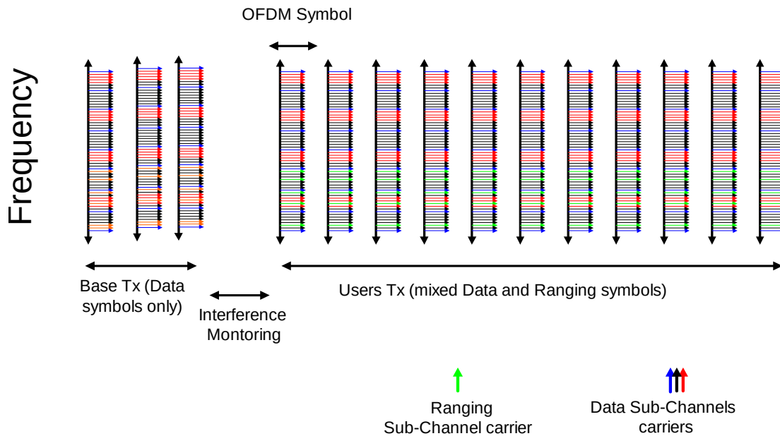
Figure 159—Ranging symbol allocation, method #2, (TDD mode)
