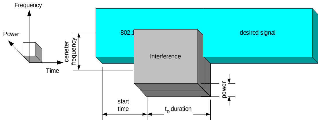
Figure 258—Interference Model
