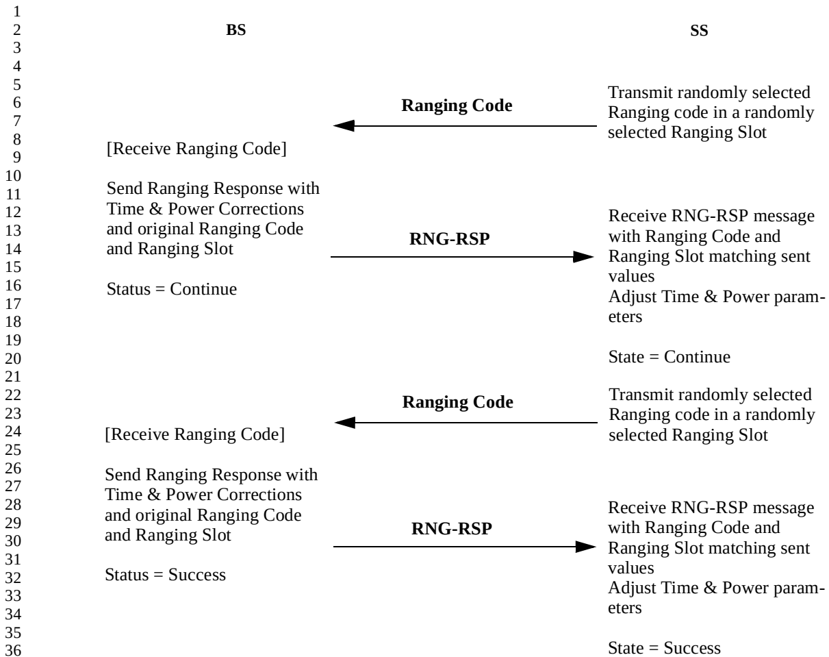
Figure 161—Ranging and automatic adjustments procedure for access scheme 2.
