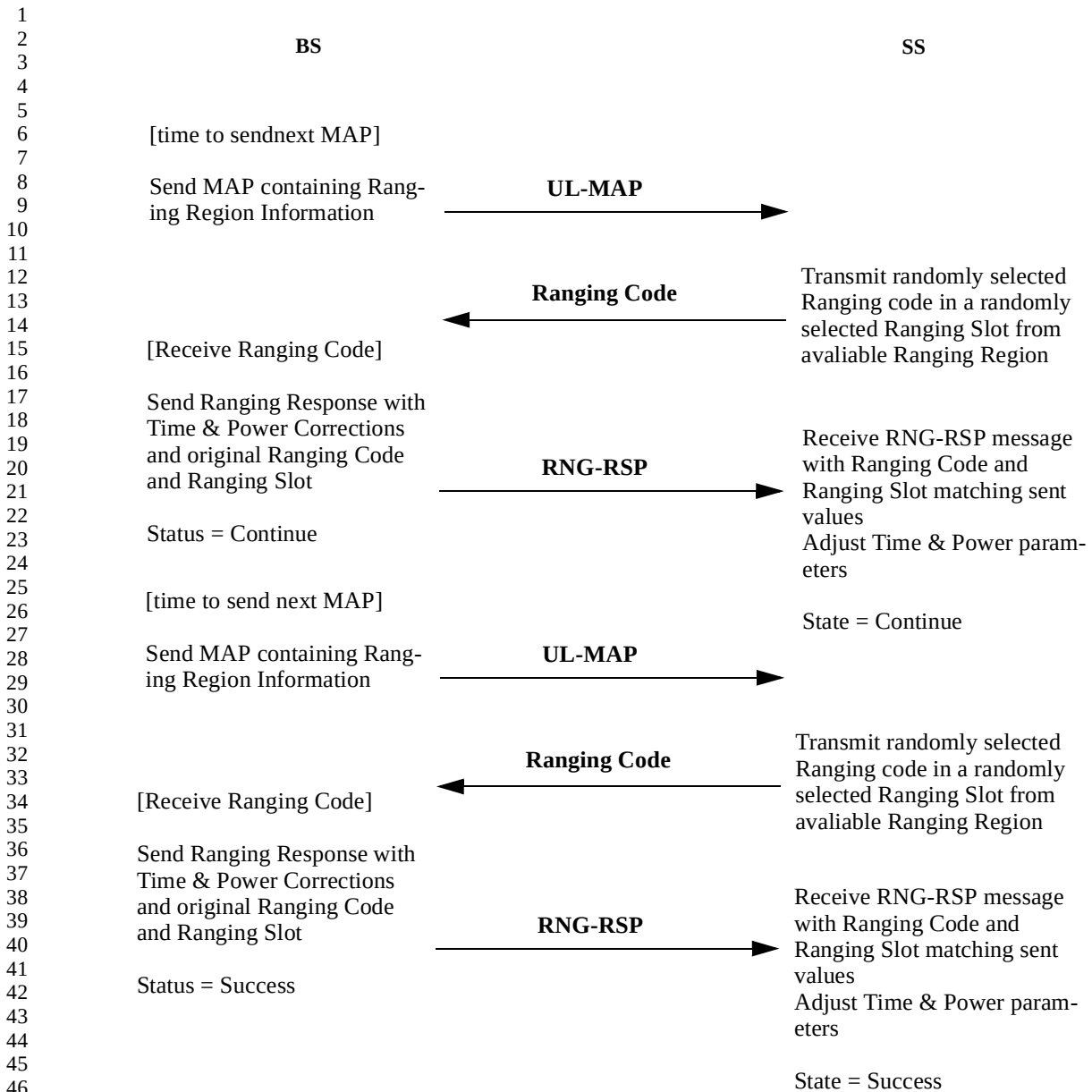
Figure 160—Ranging and automatic adjustments procedure for access scheme 1.
