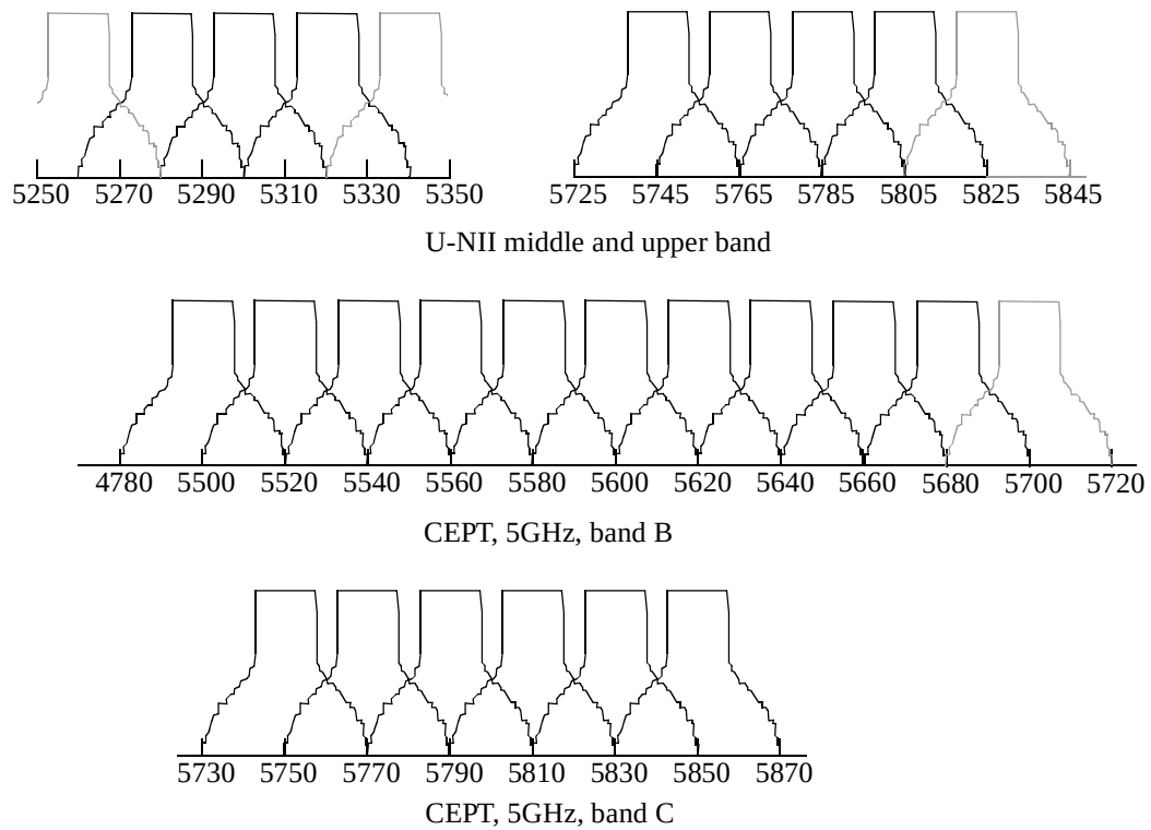
Figure 244—Channelization, 20 Mhz
