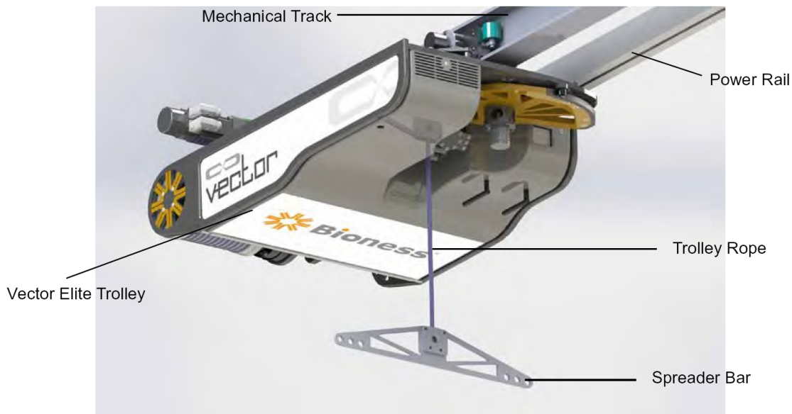
Figure 1-1: Vector Elite Trolley
