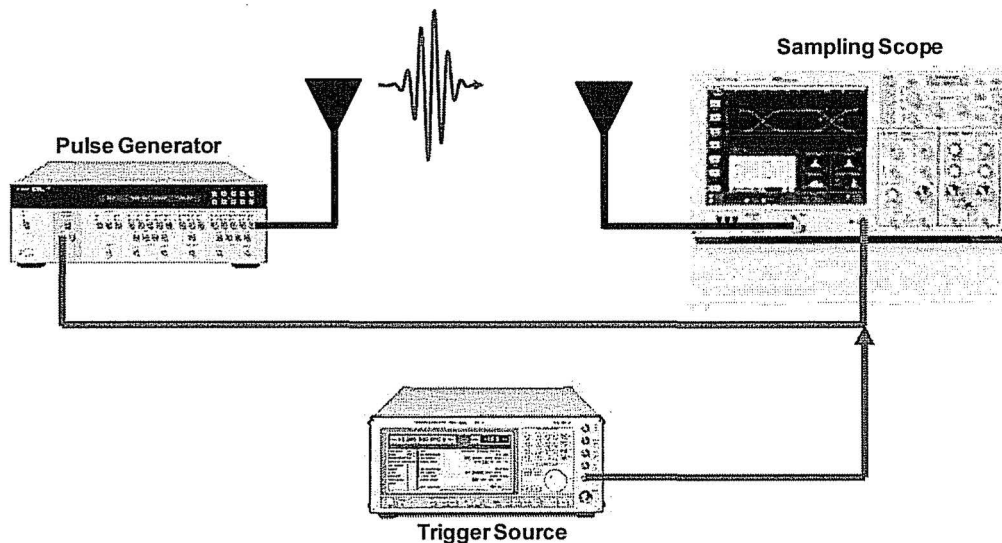
Fig. 6: Typical apparatus for capturing waveforms
