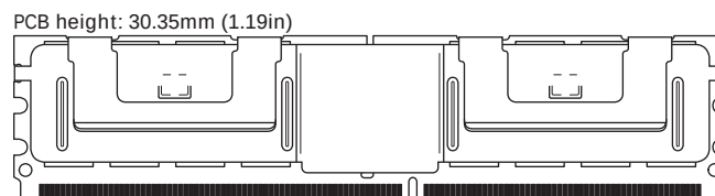
Figure 1: 240-Pin FBDIMM (MO-256)
