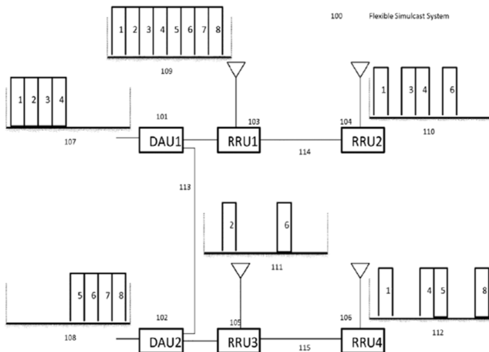
Figure 1: Flexible Simulcast Downlink Example
