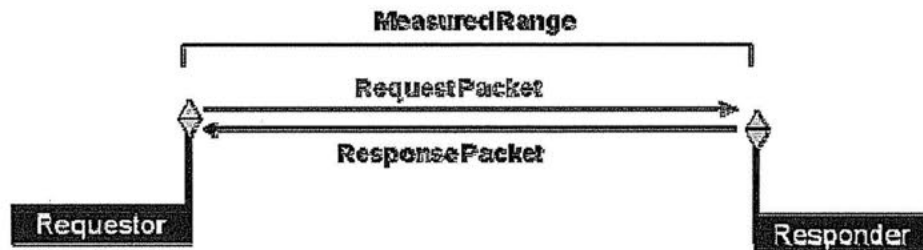
Fig. 7: Packet transmissions required by Two Way Time of Flight range measurement
