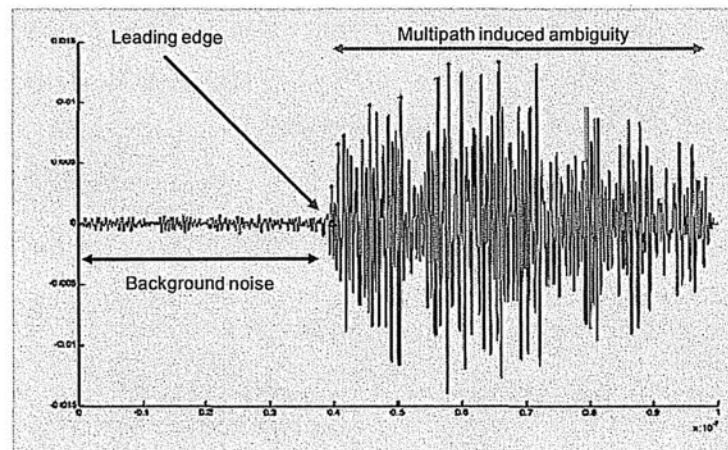
Fig. 3: Received signal in moderate multipath environment
