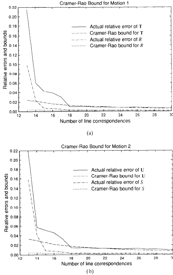
Fig. 10. Actual errors, Cramér-Rao bound for Gaussian noise versus number of line correspondences. 100 random trials: (a) Motion parameters of motion 1; (b) motion parameters of motion 2.
