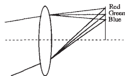
Fig.2. Lateral chromatic aberration
