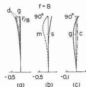
FIG. 3. Aberration curves of fish eye lens shown in Fig. 2. Curves a show spherical aberration of d and g lines and sine condition of d line, dotted. Curves b show astigmatism, and curves c show lateral color aberration for c and g lines.
