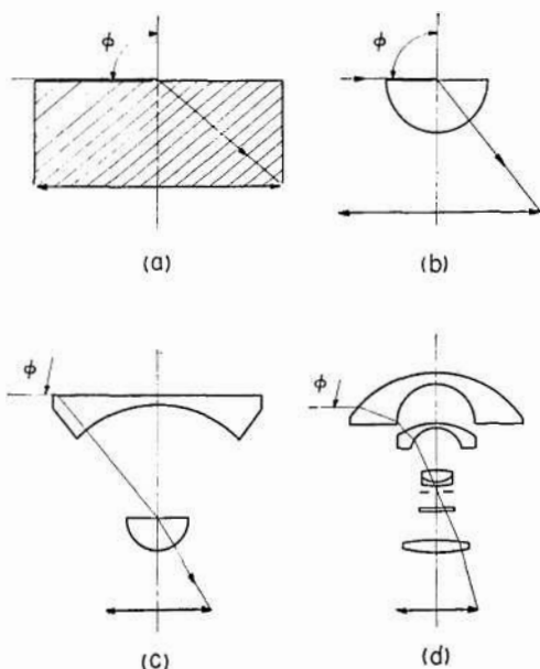
FIG. 1. Development of fish eye lens.
