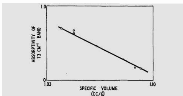
FIG. 1. Absorptivity of 73 \text{ cm}^{-1} band in polyethylene and olefin copolymers vs their specific volume.
