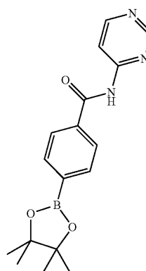
N-(Pyrimidin-4-yl)-4-(4,4,5,5-tetramethyl-1,3,2- dioxaborolan-2-yl)benzamide
