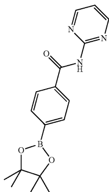
N-(Pyrimidin-2-yl)-4-(4,4,5,5-tetramethyl-1,3,2-dioxaborolan-2-yl)benzamide
