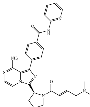
(S,E)-4-(8-Amino-3-(1-(4-(dimethylamino)but-2-enoyl)pyrrolidin-2-yl)imidazo[1,5-a]pyrazin-1-yl)-N-(pyridin-2-yl)benzamide
