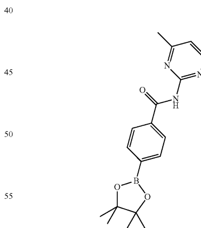
N-(4-Methylpyrimidin-2-yl)-4-(4,4,5,5-tetramethyl-1,3,2-dioxaborolan-2-yl)benzamide
