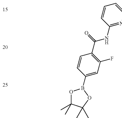
2-Fluoro-N-(pyridin-2-yl)-4-(4,4,5,5-tetramethyl-1, 3,2-dioxaborolan-2-yl)benzamide
