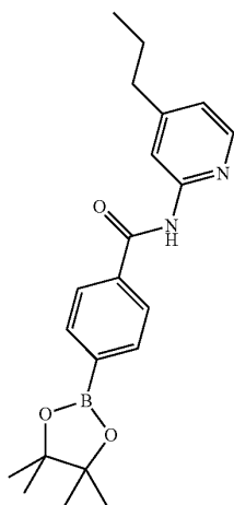
N-(4-Propylpyridin-2-yl)-4-(4,4,5,5-tetramethyl-1,3,2-dioxaborolan-2-yl)benzamide
