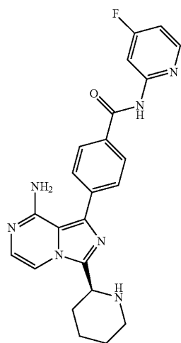
(S)-4-(8-Amino-3-(piperidin-2-yl)imidazo[1,5-a]pyrazin-1-yl)-N-(4-fluoropyridin-2-yl)benzamide
