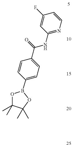
N-(4-fluoropyridin-2-yl)-4-(4,4,5,5-tetramethyl-1,3,2-dioxaborolan-2-yl)benzamide
