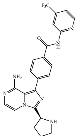
(S)-4-(8-Amino-3-(pyrrolidin-2-yl)imidazo[1,5-a]pyrazin-1-yl)-N-(4-(trifluoromethyl)pyridin-2-yl)benzamide
