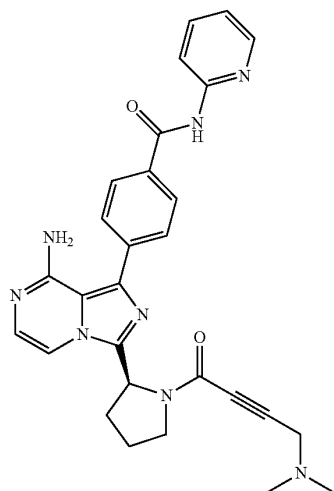
(S)-4-(8-Amino-3-(1-(4-(dimethylamino)but-2-ynoyl)pyrrolidin-2-yl)imidazo[1,5-a]pyrazin-1-yl)-N-(pyridin-2-yl)benzamide
