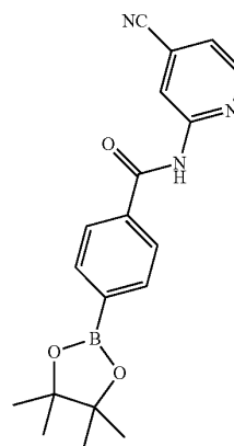
N-(4-Cyanopyridin-2-yl)-4-(4,4,5,5-tetramethyl-1,3,2-dioxaborolan-2-yl)benzamide
