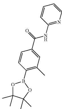
3-Methyl-N-(pyridin-2-yl)-4-(4,4,5,5-tetramethyl-1,3,2-dioxaborolan-2-yl)benzamide
