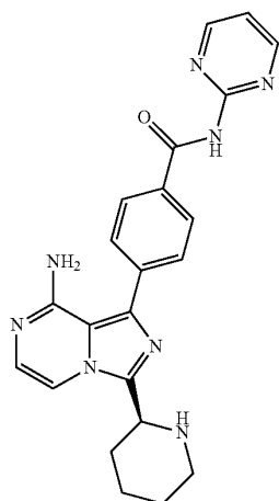
(S)-4-(8-Amino-3-(piperidin-2-yl)imidazo[1,5-a]pyrazin-1-yl)-N-(pyrimidin-2-yl)benzamide
