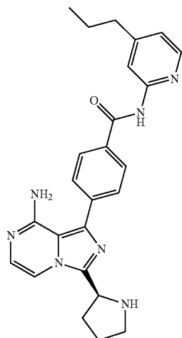
(S)-4-(8-Amino-3-(pyrrolidin-2-yl)imidazo[1,5-a]pyrazin-1-yl)-N-(4-propylpyridin-2-yl)benzamide
