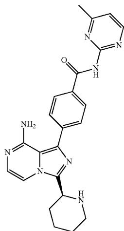
(S)-4-(8-Amino-3-(piperidin-2-yl)imidazo[1,5-a] pyrazin-1-yl)-N-(4-methylpyrimidin-2-yl)benzamide
