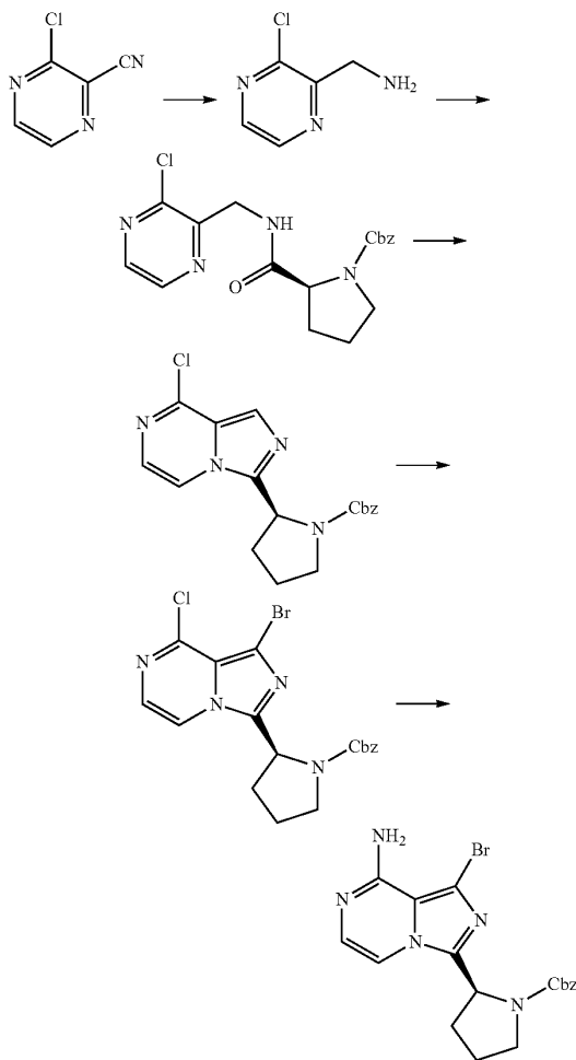
(S)-Benzyl 2-((8-amino-1-bromoimidazo[1,5-a]pyrazin-3-yl)pyrrolidine-1-carboxylate
