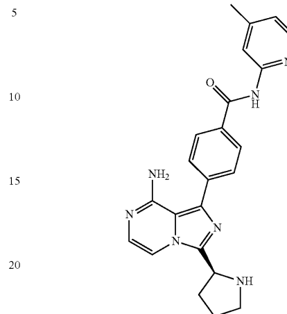
(S)-4-(8-Amino-3-(pyrrolidin-2-yl)imidazo[1,5-a]pyrazin-1-yl)-N-(4-methylpyridin-2-yl)benzamide
