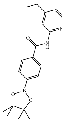
N-(4-Ethylpyridin-2-yl)-4-(4,4,5,5-tetramethyl-1,3,2-dioxaborolan-2-yl)benzamide
