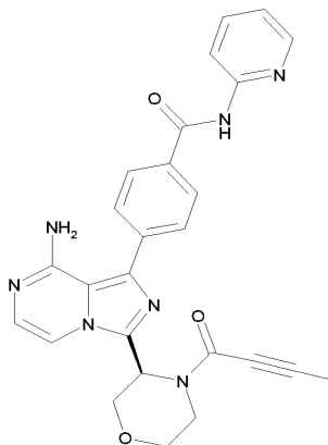
(R)-4-(8-Amino-3-(4-but-2-ynoylmorpholin-3-yl)imidazo[1,5-a]pyrazin-1-yl)-N-(pyridin-2-yl)benzamide
