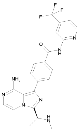
(S)-4-(8-Amino-3-(1-(methilamino)ethyl)imidazo[1,5-a]pyrazin-1-yl)-N-(4-(trifluoromethyl)pyridin-2-yl)benzamide
