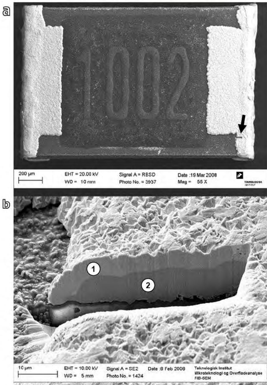
Fig. 5.9: SEM micrographs of chip resistor: (a) Top side of resistor with FIB cross section (marked by arrow) and (b) High magnification of FIB cross section revealing Sn layer (1) with Ni under layer (2).
