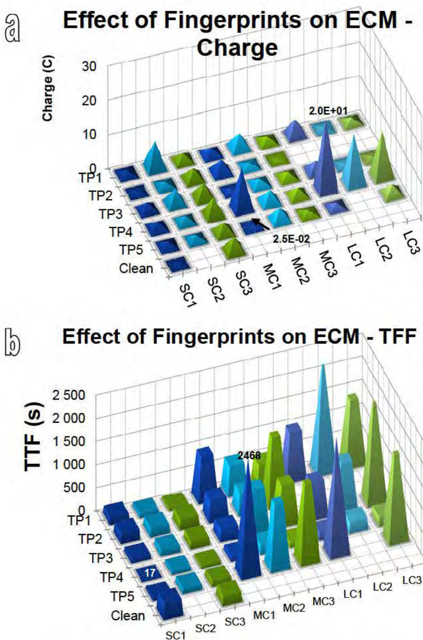
Figure 9.16: a) Charge and b) TFF plots showing the effect of fingerprints from 5 different test persons (TP) on migration. Minimum and maximum values are shown in both diagrams.
