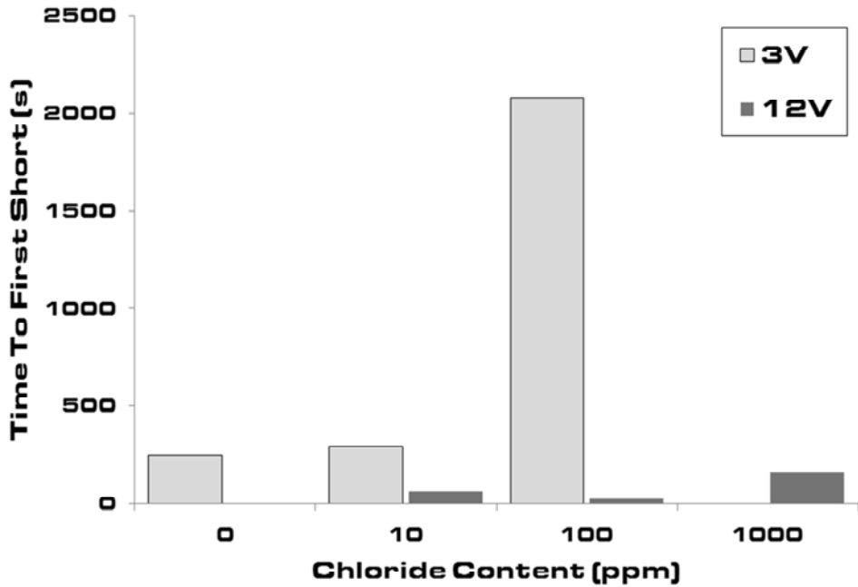
Fig. 5.17: Time for first short circuit due to electrochemical migration for 3V and 12V at varying sodium chloride concentrations.
