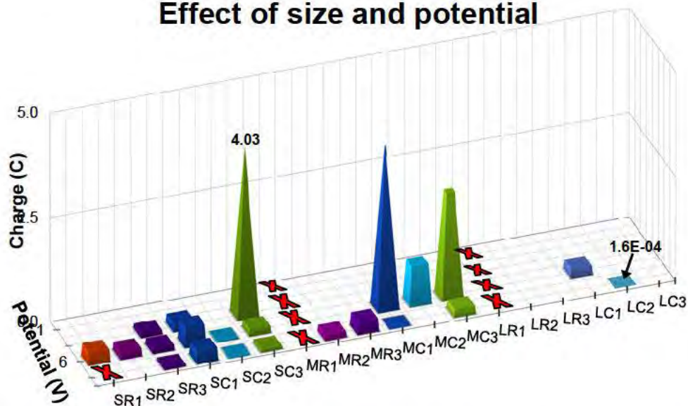
Figure 9.12: Plot showing the effect of size of component and potential on the ECM susceptibility on PCB represented by the total charge passed during dendrite formation and shorting. Values for minimum (LC2-18V) and maximum (SC3-3V) are shown in Coulombs.
