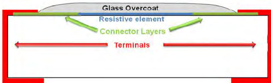
Fig. 5.6: Schematic of Surface mount chip resistor material make-up.
