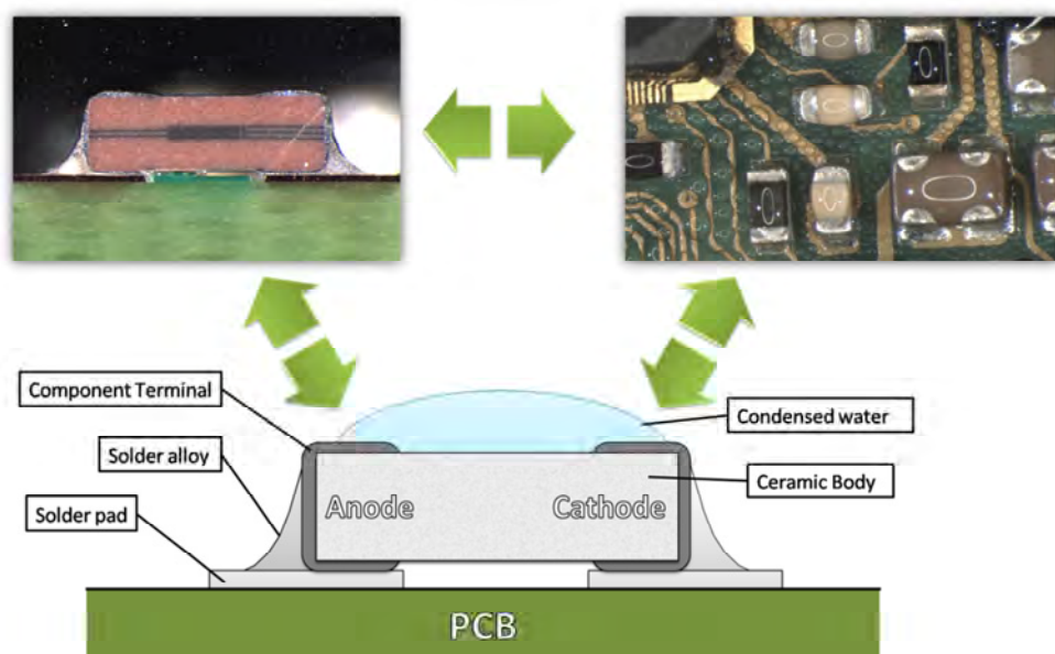
Figure 8.2: Sketch presenting an example of condensation on a PCBA, a cross section of an SMD chip capacitor on a PCBA, and a simplified sketch showing the material makeup.
