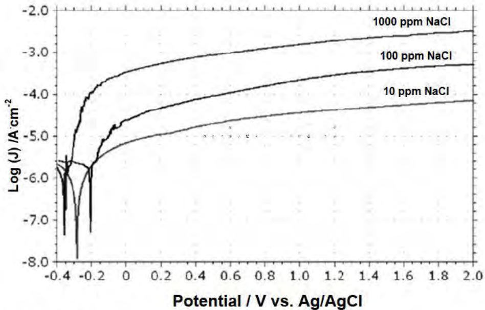
Fig. 5.10: Anodic polarization curves for solder terminals on ceramic chip resistor. The Y-axis is showing the logarithm to the current density (J) and the X-axis has the potential vs. Ag/AgCl reference electrode (215 mV vs. SHE).
