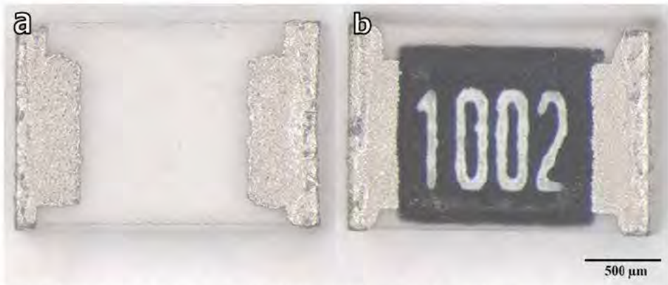
Fig. 5.5: Ceramic chip resistor with size 0805 used in this work: (a) bottom side and (b) top side. Resistance of the component is 10 kΩ.
