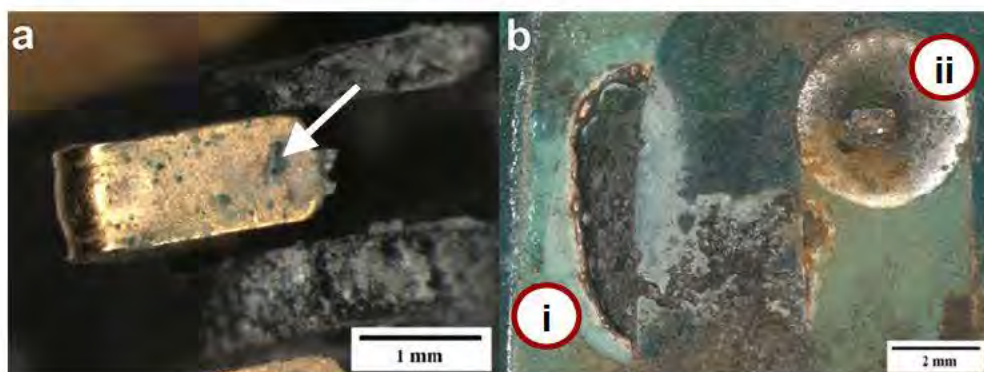
Figure 1.2: a) Example of corrosion of Ni underlayer on an ENIG contact due to galvanic cell formation between Ni anode and Au cathode. Green Ni corrosion products can be seen protruding from the gold layer, as indicated by the arrow. b) Electrolytic corrosion between Cu conducting line which is coated by soldermask (i) and Sn soldered through hole component (ii) on a PCB due to humidity ingress through soldermask coating. Both failures are from testing in harsh environment.
