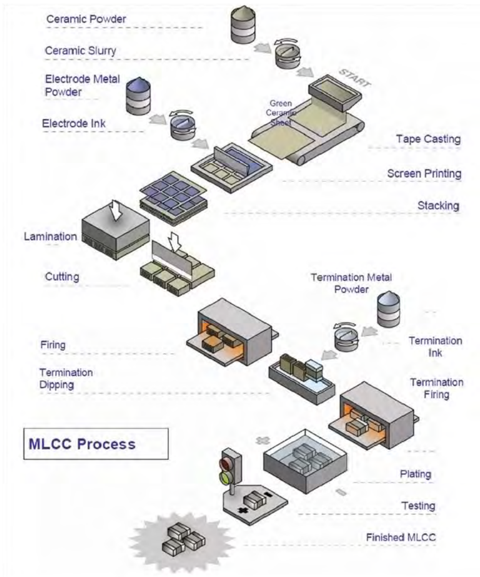
Figure 2.8: Example of the manufacturing process for multilayer ceramic chip capacitors (MLCC) (Reprinted with permission from Johanson Dielectrics, CA, USA)
