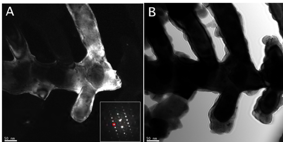
Figure 6.12: A) Dark field and B) bright field images, obtained from the (\bar{2}11) direction as indicated by the red circle on the diffraction pattern (insert in image A. Orientation is along the [1,1,3] zone axis (see Figure 6.10F)). Dendrite branch is from the location shown in Figure 6.9D (12V sample).
