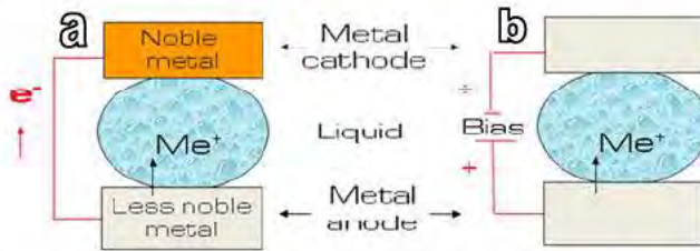
Fig. 5.1: Two possibilities for corrosion cell formation on a PCB with condensed electrolyte: (a) Galvanic coupling due to different materials on PCB and (b) Formation of electrochemical cell between similar electrodes due to applied bias.
