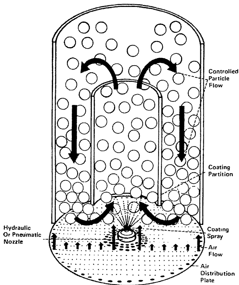
Fig. 25 Diagram of Wurster coating chamber.
