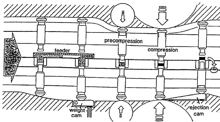
Fig. 15 Multistation press cycle.
