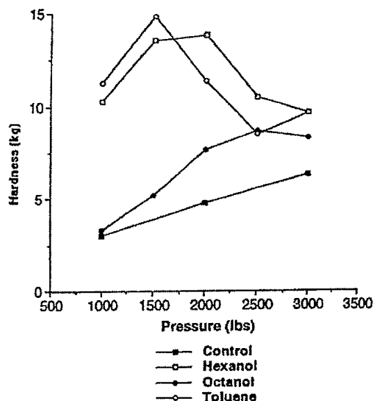
Fig. 3 Intrinsic compressibility of nonagglomerated naproxen (control) and of naproxen that has been spherically agglomerated with different solvents. (From Ref. 21.)
