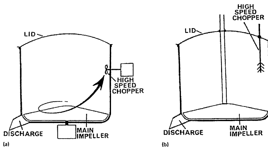
Fig. 13 High-shear mixers: (a) underdriven; (b) overdriven.
