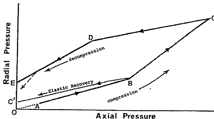
Fig. 19 Compaction profile.
