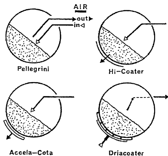
Fig. 24 Coating pan air configurations.
