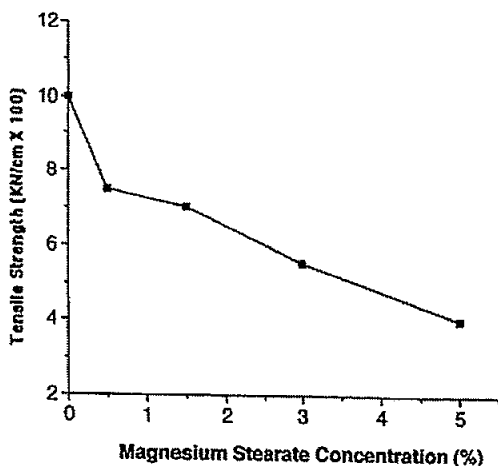
Fig. 12 Tensile strength of calcium sulfate tablets as a function of magnesium stearate concentration (solid fraction = 0.57). (From Ref. 29.)
