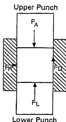
Fig. 14 Forces developed in the formation of a tablet compact. ▨, die wall; F_A , axial pressure applied by upper punch; F_D , force lost to die wall; F_R , radial die wall; □, tablet compact.
