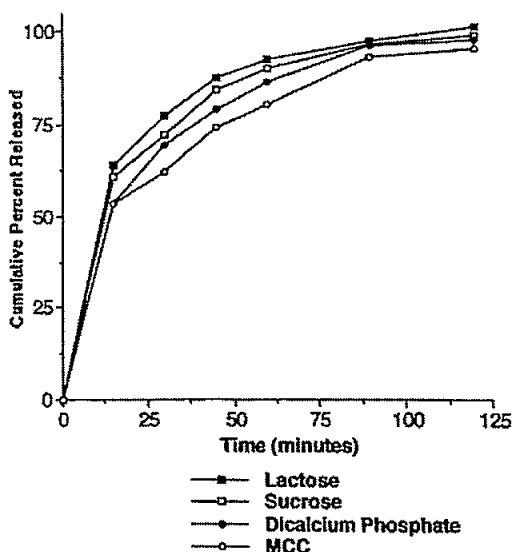
Fig. 6 Dissolution of digoxin tablets containing different fillers (in simulated gastric fluid at 37°C). (From Ref. 45.)
