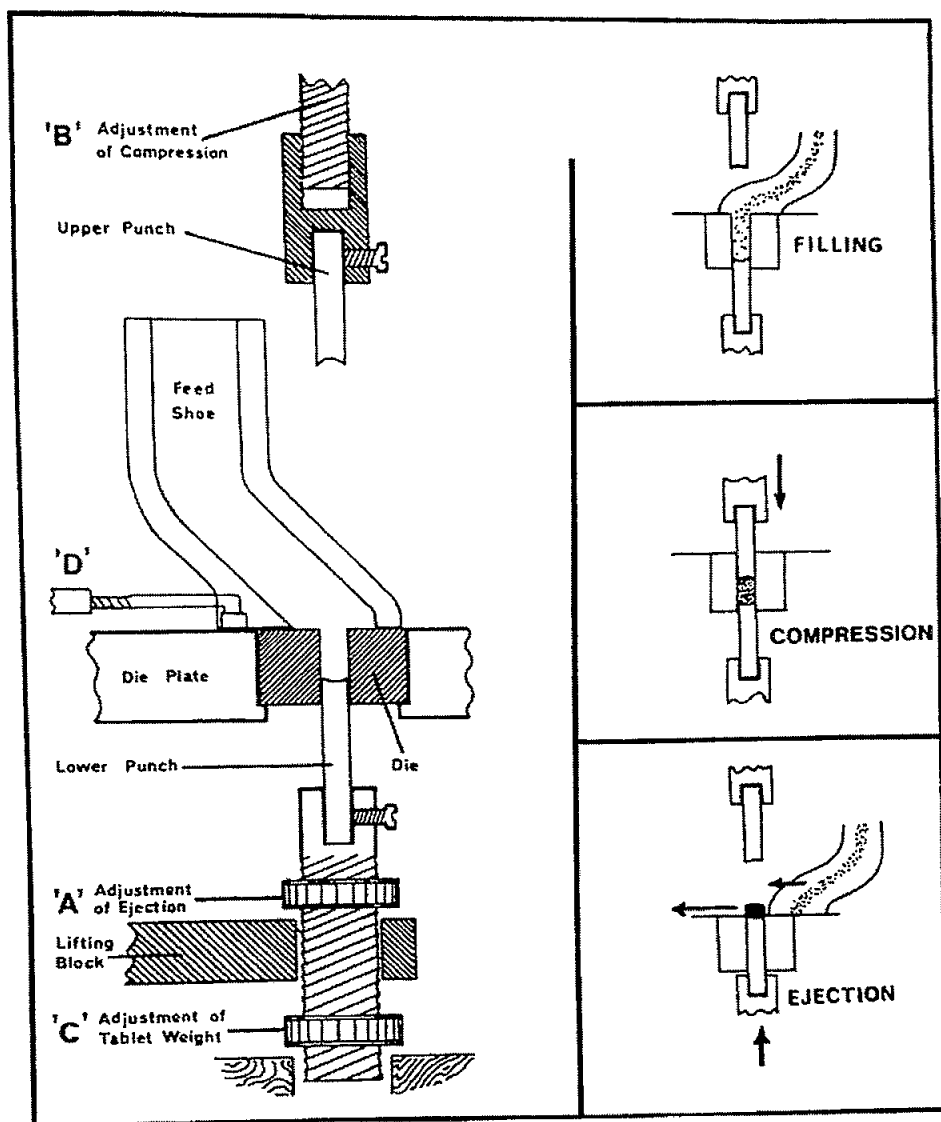
Fig. 16 Single station press cycle.
