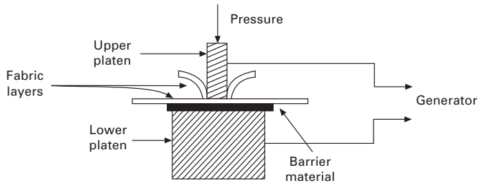
12.6 A typical dielectric welding machine.
