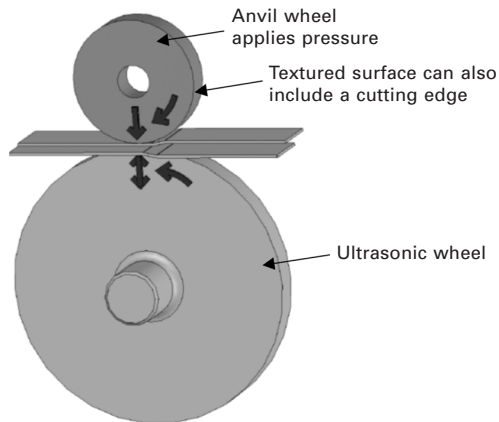
12.3 Continuous ultrasonic wheel welding.
