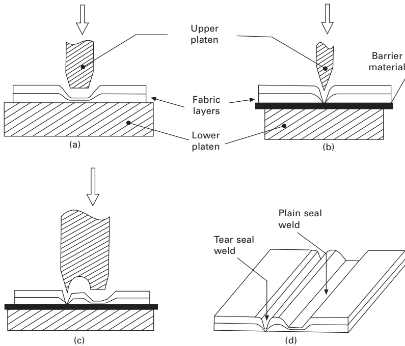
12.7 Types of dielectric welding: (a) plain-seal welding; (b) tear-seal welding; (c) combined plain and tear-seal welding; (d) combined weld from (c).
