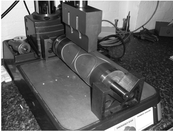
12.4 Continuous ultrasonic drum welding machine.
