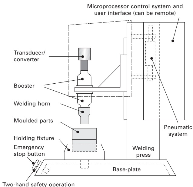
12.1 Schematic of a typical ultrasonic plunge welding machine.
