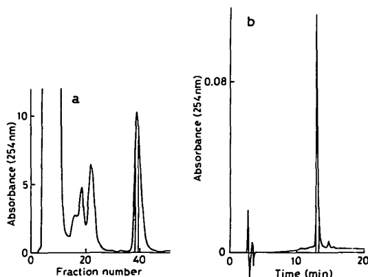
Fig. 1 a) Reversed phase chromatography of 5'-dimethoxytrityl 9 mer (AmCmUmUmAmCmCmUmGm) using a column (0.7 x 12 cm) of C-18 silica gel (35-105 u, Waters Associates) with a linear gradient of acetonitrile (5-35%) in 50 mM triethylammonium bicarbonate (total, 200 ml). Fractions of 3 ml were collected every 4 min. b) Reversed phase HPLC of the dedimethoxytritylated 9 mer (fraction 38) using a column (0.46 x 30 cm) of Nucleosil 5C 18 (Macherey-Nagel) with a linear gradient of acetonitrile (from 13 to 21% during 20 min) in 0.1 M triethylammonium acetate. The flow rate was 1 ml/min.
